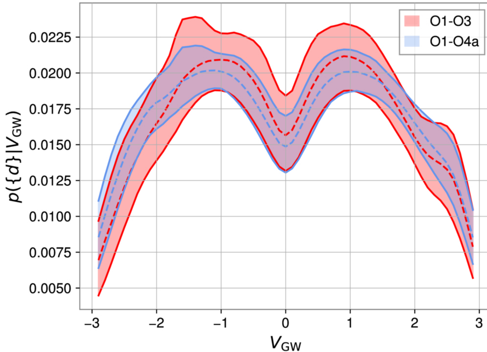
Figure 5. from Juan Calderón Bustillo et al 2026 Astrophys. J. Lett. 1008 doi:10.3847/2041-8213/ae9740 https://dx.doi.org/10.3847/2041-8213/ae9740 © 2026. The Author(s). Published by the American Astronomical Society.
