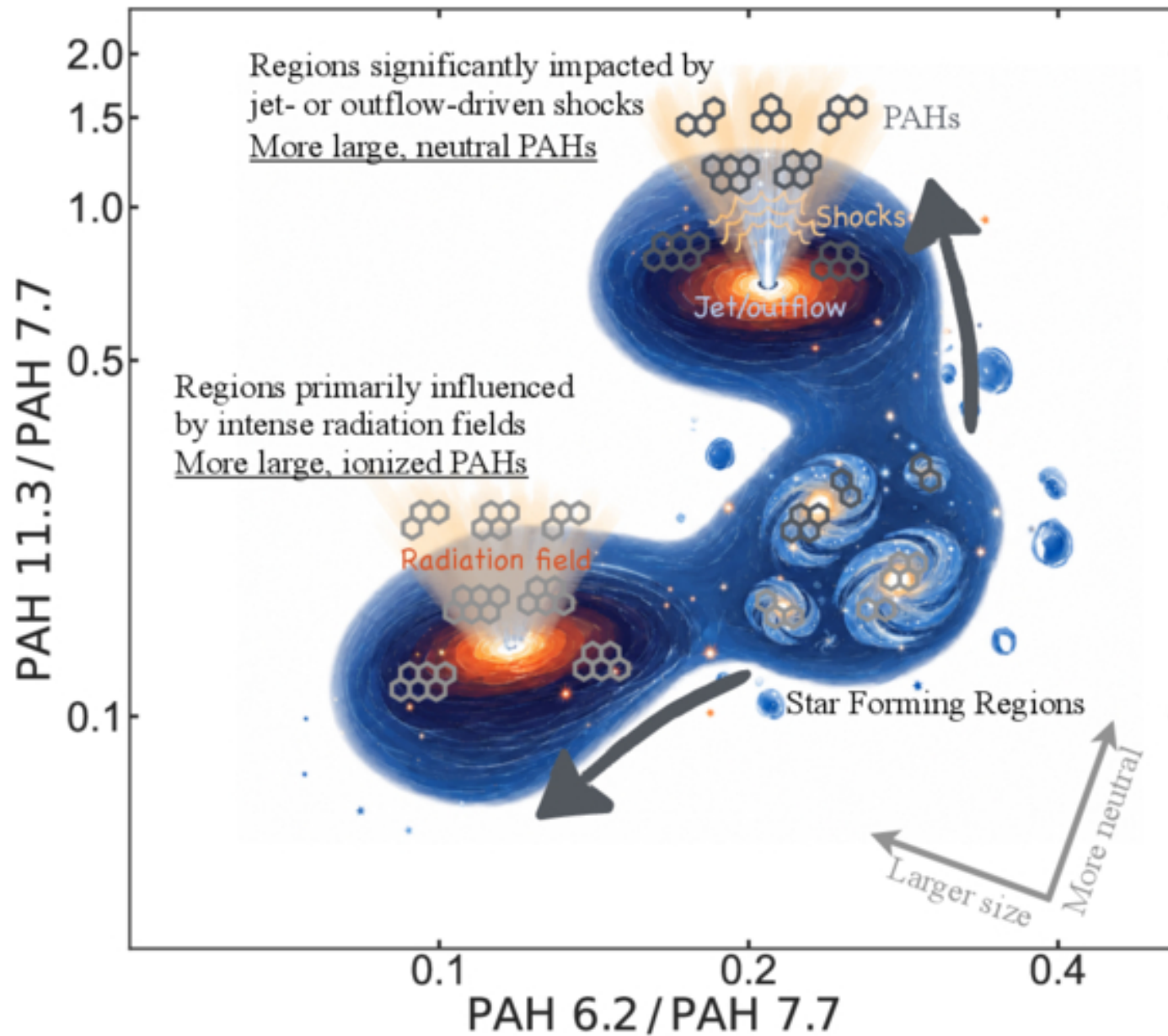
Figure 6. from Lulu Zhang et al 2026 Astrophys. J. Lett. 1007 doi:10.3847/2041-8213/ae96b6 https://dx.doi.org/10.3847/2041-8213/ae96b6 © 2026. The Author(s). Published by the American Astronomical Society.
