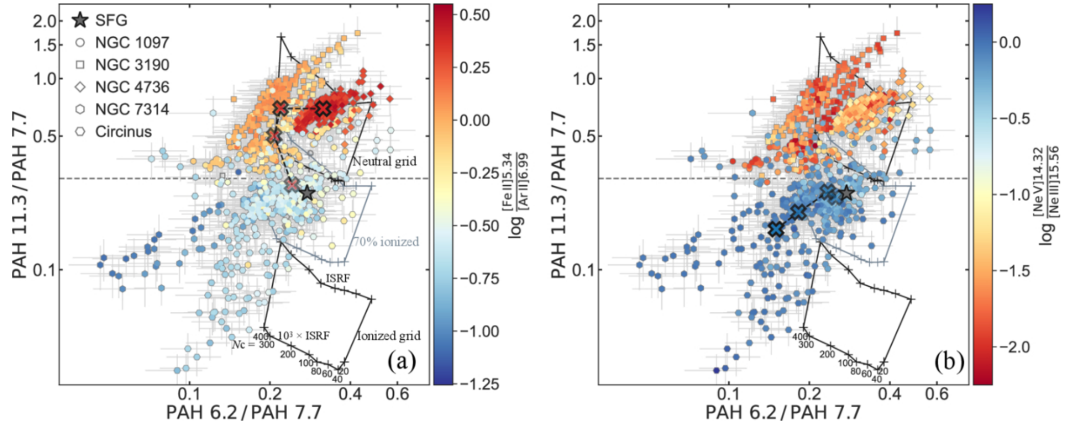
Figure 5. from Lulu Zhang et al 2026 Astrophys. J. Lett. 1007 doi:10.3847/2041-8213/ae96b6 https://dx.doi.org/10.3847/2041-8213/ae96b6 © 2026. The Author(s). Published by the American Astronomical Society.
