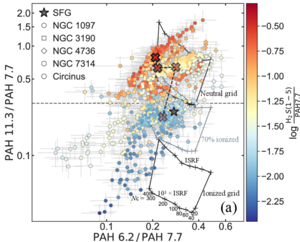
Figure 4. from Lulu Zhang et al 2026 Astrophys. J. Lett. 1007 doi:10.3847/2041-8213/ae96b6 https://dx.doi.org/10.3847/2041-8213/ae96b6 © 2026. The Author(s). Published by the American Astronomical Society.
