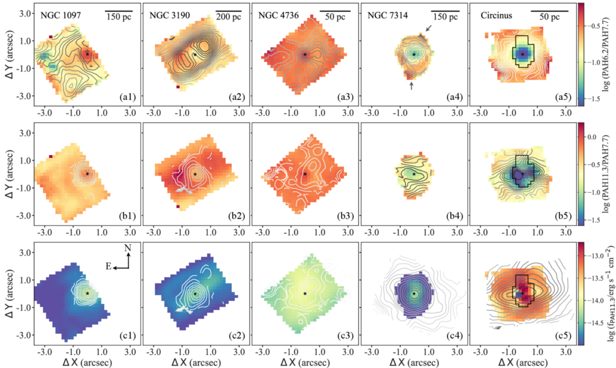
Figure 3. from Lulu Zhang et al 2026 Astrophys. J. Lett. 1007 doi:10.3847/2041-8213/ae96b6 https://dx.doi.org/10.3847/2041-8213/ae96b6 © 2026. The Author(s). Published by the American Astronomical Society.
