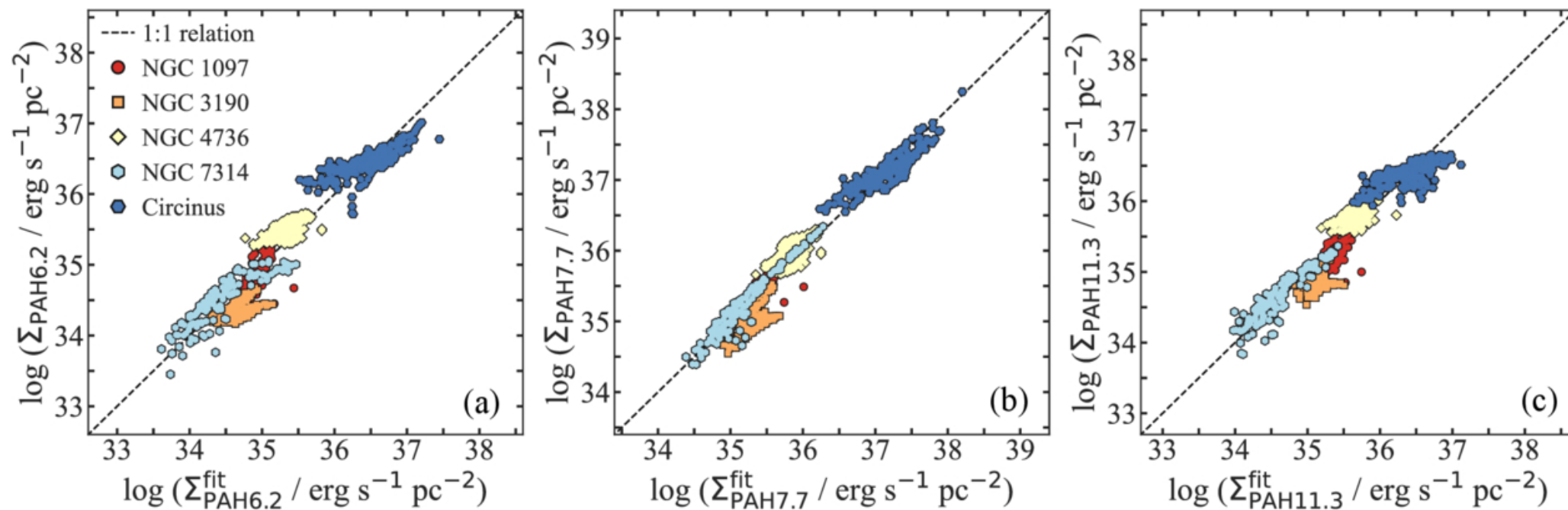
Figure 2. from Lulu Zhang et al 2026 Astrophys. J. Lett. 1007 doi:10.3847/2041-8213/ae96b6 https://dx.doi.org/10.3847/2041-8213/ae96b6 © 2026. The Author(s). Published by the American Astronomical Society.
