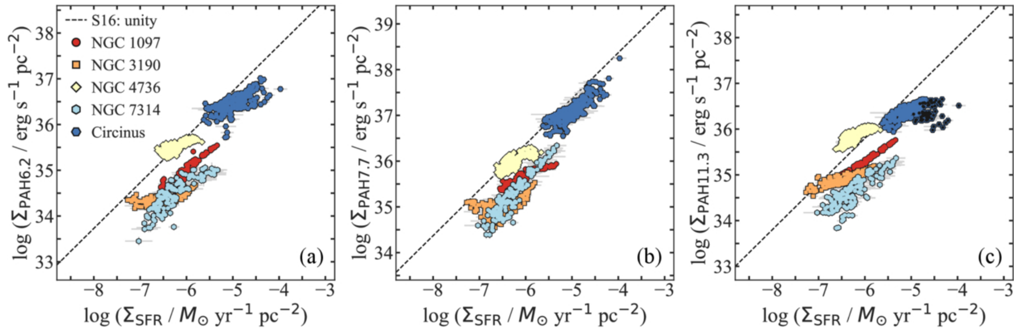
Figure 1. from Lulu Zhang et al 2026 Astrophys. J. Lett. 1007 doi:10.3847/2041-8213/ae96b6 https://dx.doi.org/10.3847/2041-8213/ae96b6 © 2026. The Author(s). Published by the American Astronomical Society.
