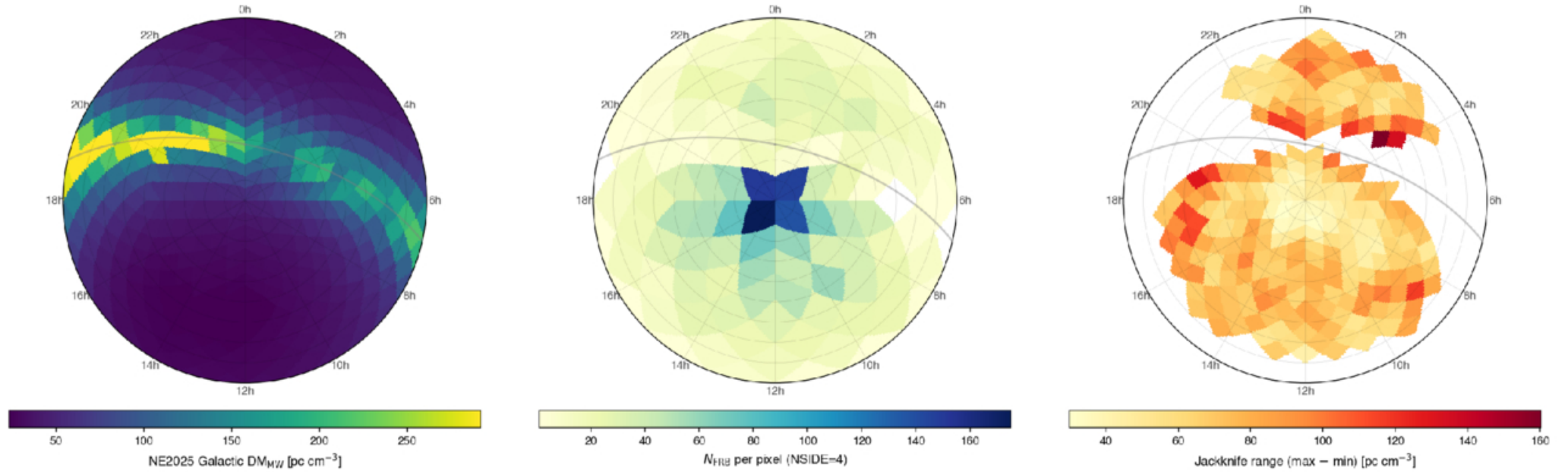
Figure 3. from Vikram Ravi et al 2026 Astrophys. J. Lett. 1008 doi:10.3847/2041-8213/ae96b0 https://dx.doi.org/10.3847/2041-8213/ae96b0 © 2026. The Author(s). Published by the American Astronomical Society.
