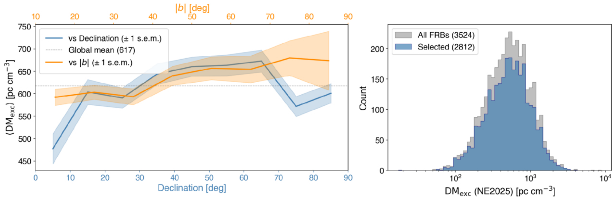
Figure 1. from Vikram Ravi et al 2026 Astrophys. J. Lett. 1008 doi:10.3847/2041-8213/ae96b0 https://dx.doi.org/10.3847/2041-8213/ae96b0 © 2026. The Author(s). Published by the American Astronomical Society.
