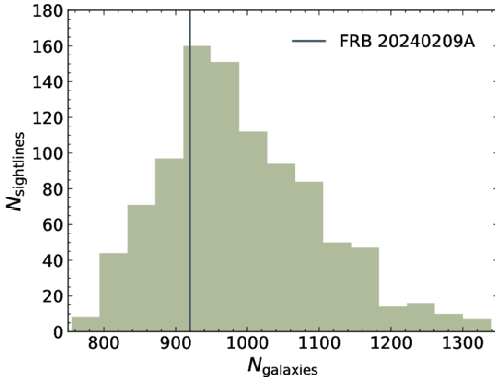
Figure 9. from Samuel McCarty et al 2026 Astrophys. J. Lett. 1007 doi:10.3847/2041-8213/ae96af https://dx.doi.org/10.3847/2041-8213/ae96af © 2026. The Author(s). Published by the American Astronomical Society.
