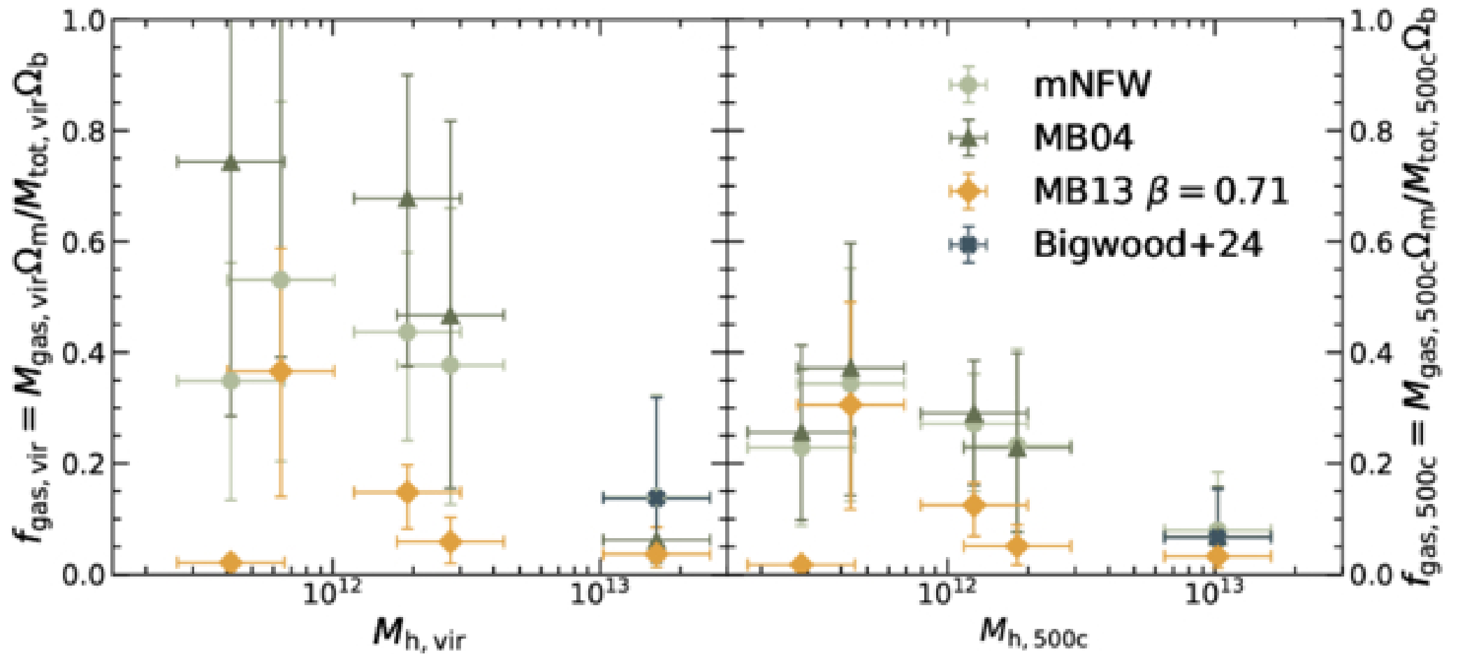
Figure 6. from Samuel McCarty et al 2026 Astrophys. J. Lett. 1007 doi:10.3847/2041-8213/ae96af https://dx.doi.org/10.3847/2041-8213/ae96af © 2026. The Author(s). Published by the American Astronomical Society.
