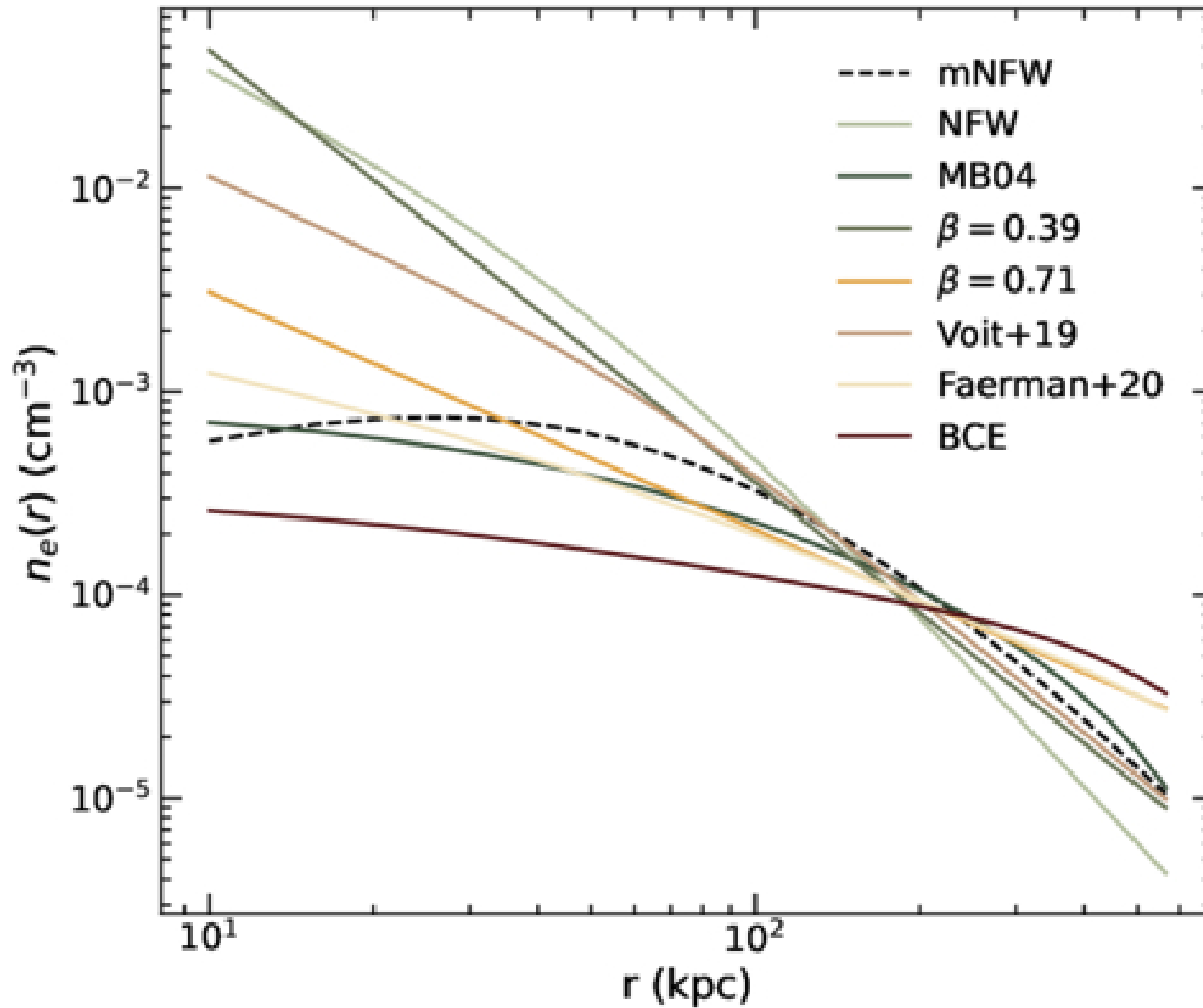
Figure 5. from Samuel McCarty et al 2026 Astrophys. J. Lett. 1007 doi:10.3847/2041-8213/ae96af https://dx.doi.org/10.3847/2041-8213/ae96af © 2026. The Author(s). Published by the American Astronomical Society.
