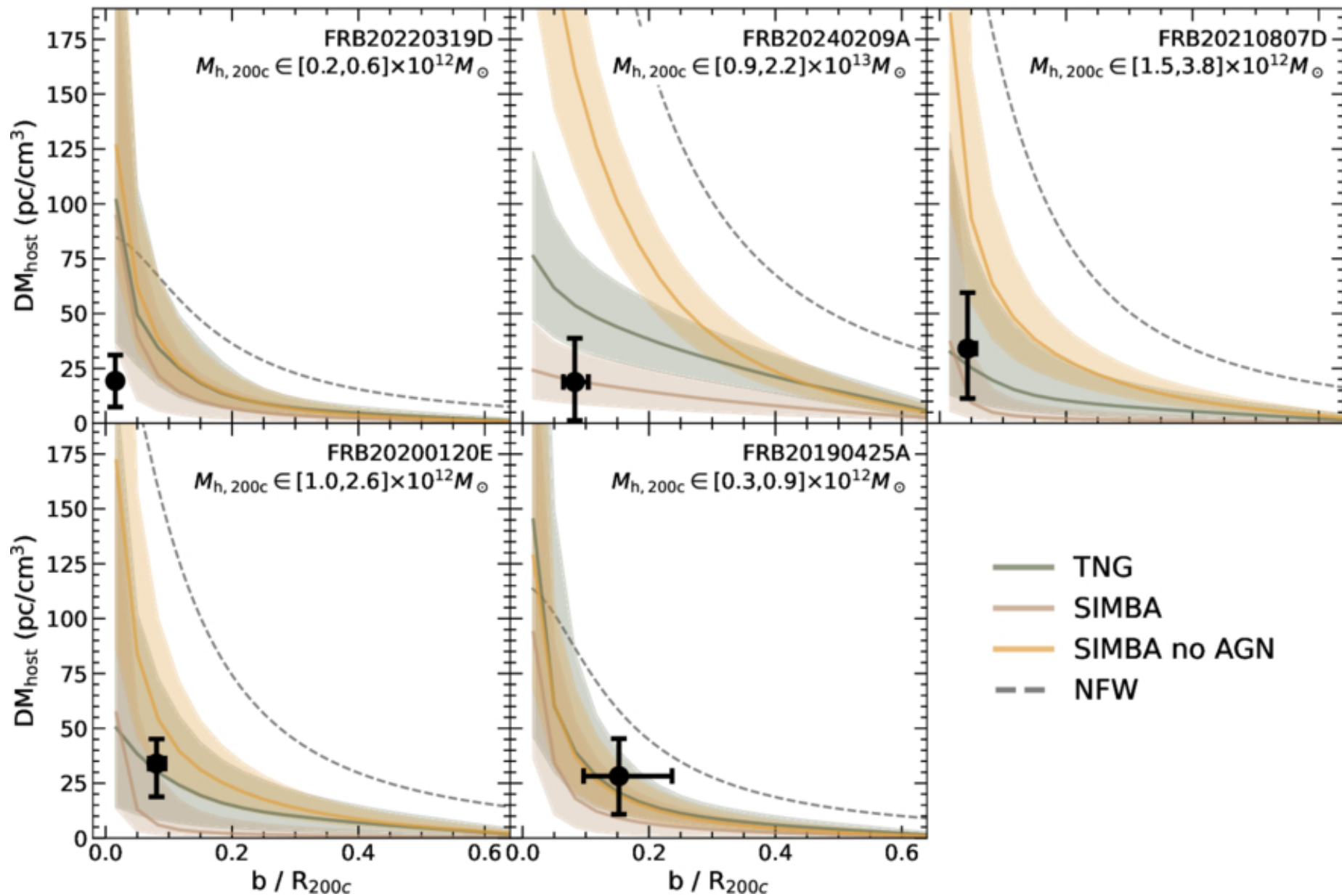
Figure 4. from Samuel McCarty et al 2026 Astrophys. J. Lett. 1007 doi:10.3847/2041-8213/ae96af https://dx.doi.org/10.3847/2041-8213/ae96af © 2026. The Author(s). Published by the American Astronomical Society.
