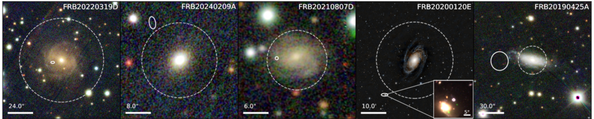
Figure 2. from Samuel McCarty et al 2026 Astrophys. J. Lett. 1007 doi:10.3847/2041-8213/ae96af https://dx.doi.org/10.3847/2041-8213/ae96af © 2026. The Author(s). Published by the American Astronomical Society.
