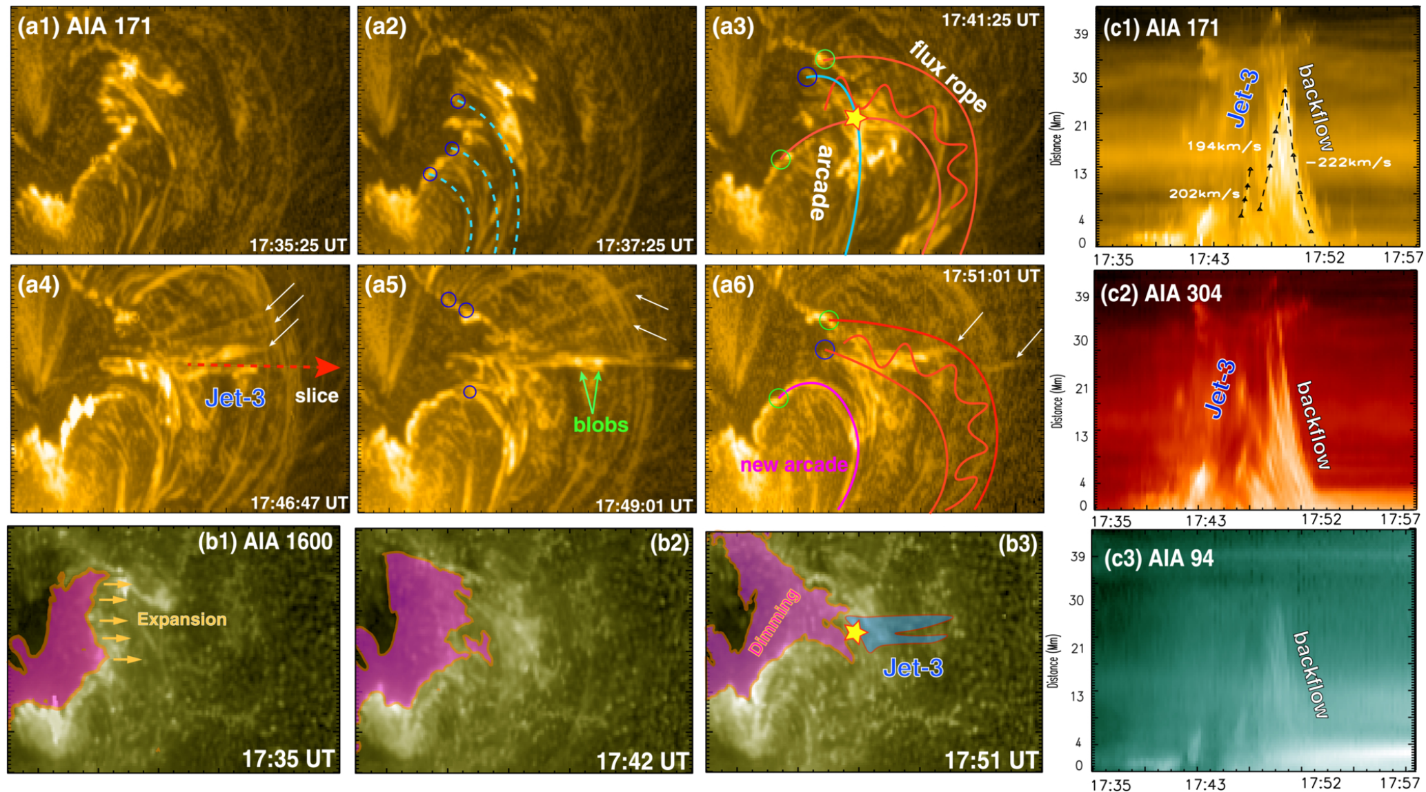
Figure 4. from Renjie Liu et al 2026 Astrophys. J. Lett. 1008 doi:10.3847/2041-8213/ae969a https://dx.doi.org/10.3847/2041-8213/ae969a © 2026. The Author(s). Published by the American Astronomical Society.
