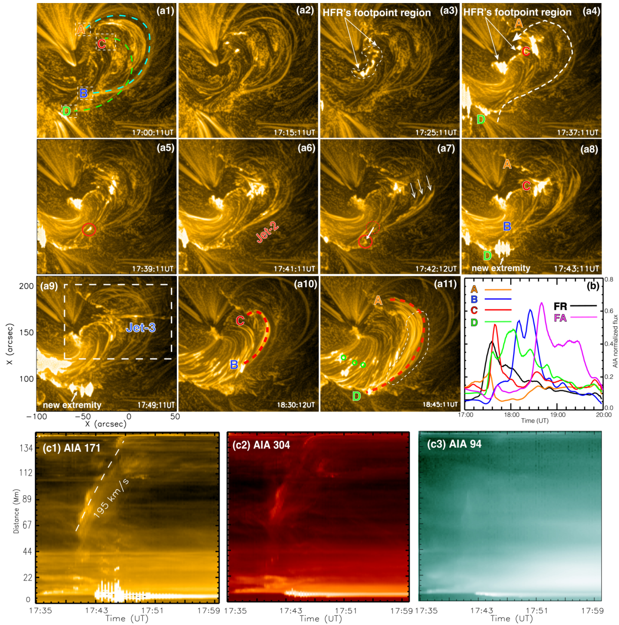
Figure 3. from Renjie Liu et al 2026 Astrophys. J. Lett. 1008 doi:10.3847/2041-8213/ae969a https://dx.doi.org/10.3847/2041-8213/ae969a © 2026. The Author(s). Published by the American Astronomical Society.
