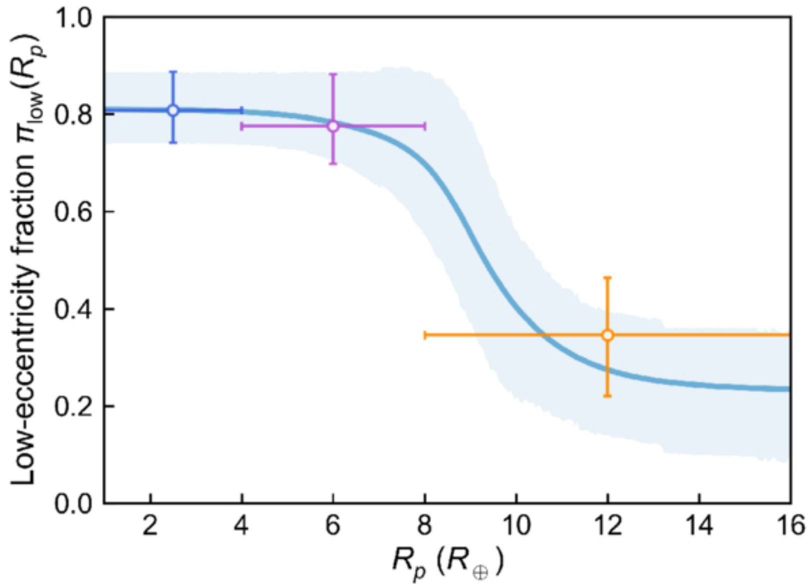
Figure 7. from Tyler R. Fairnington et al 2026 Astrophys. J. Lett. 1008 doi:10.3847/2041-8213/ae9612 https://dx.doi.org/10.3847/2041-8213/ae9612 © 2026. The Author(s). Published by the American Astronomical Society.
