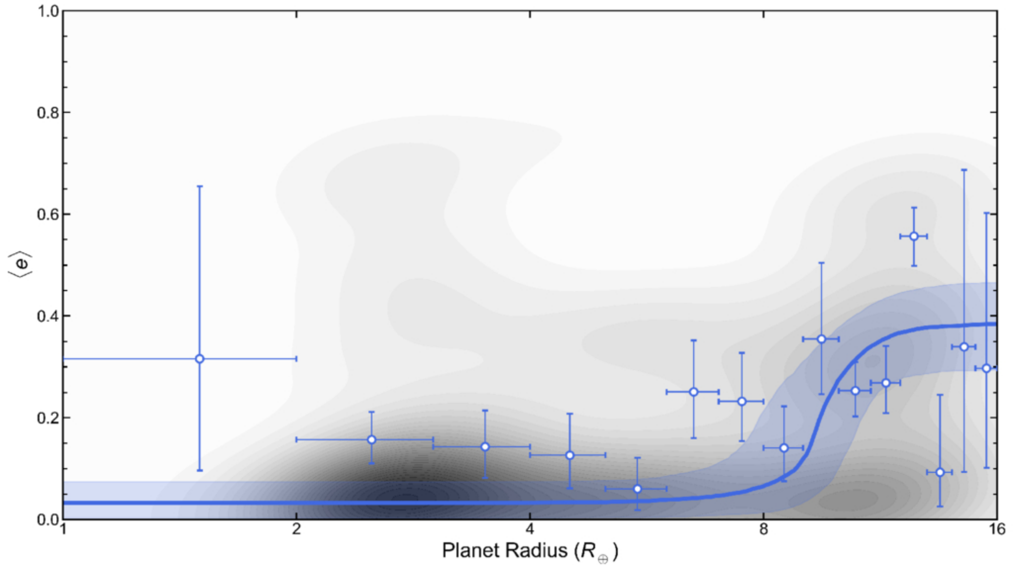
Figure 6. from Tyler R. Fairnington et al 2026 Astrophys. J. Lett. 1008 doi:10.3847/2041-8213/ae9612 https://dx.doi.org/10.3847/2041-8213/ae9612 © 2026. The Author(s). Published by the American Astronomical Society.
