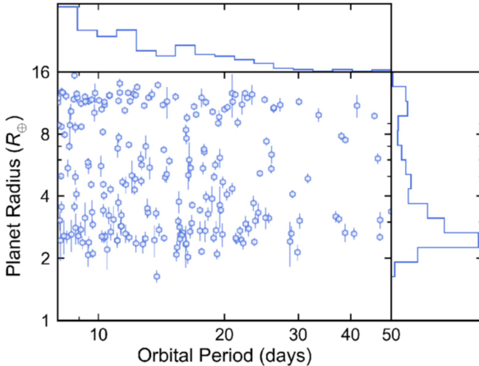
Figure 1. from Tyler R. Fairnington et al 2026 Astrophys. J. Lett. 1008 doi:10.3847/2041-8213/ae9612 https://dx.doi.org/10.3847/2041-8213/ae9612 © 2026. The Author(s). Published by the American Astronomical Society.
