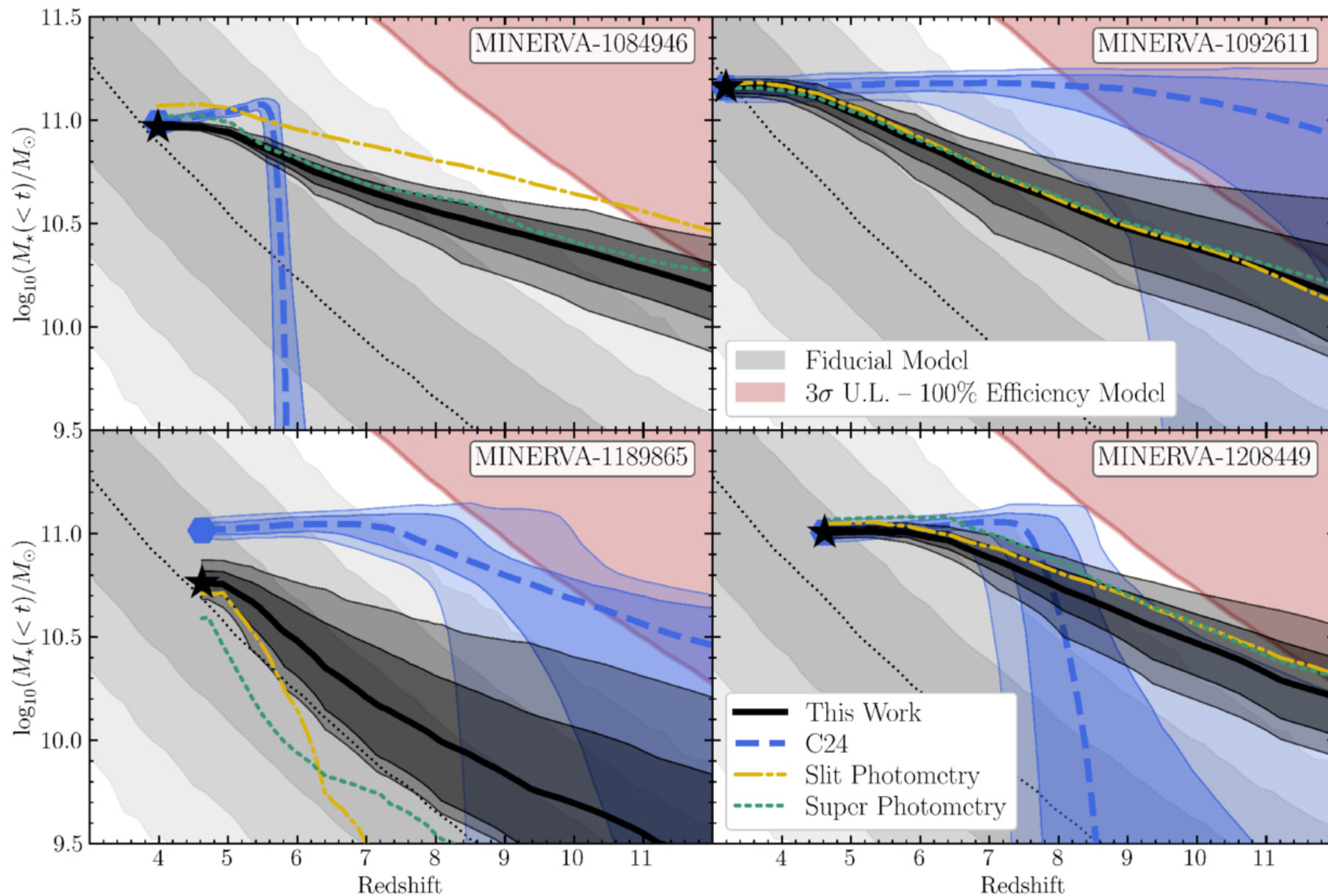
Figure 5. from Sam E. Cutler et al 2026 Astrophys. J. Lett. 1008 doi:10.3847/2041-8213/ae960c https://dx.doi.org/10.3847/2041-8213/ae960c © 2026. The Author(s). Published by the American Astronomical Society.
