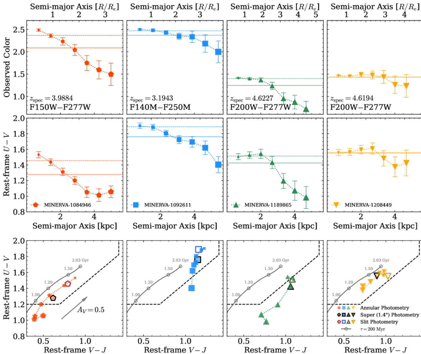
Figure 2. from Sam E. Cutler et al 2026 Astrophys. J. Lett. 1008 doi:10.3847/2041-8213/ae960c https://dx.doi.org/10.3847/2041-8213/ae960c
