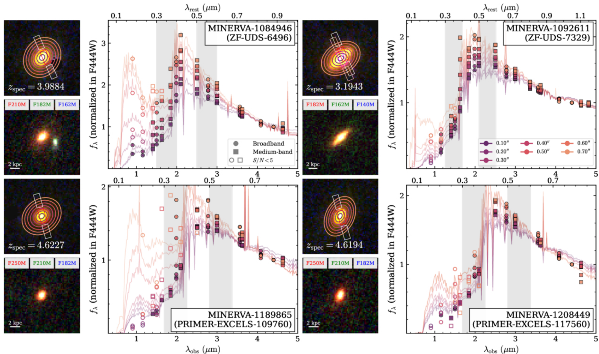
Figure 1. from Sam E. Cutler et al 2026 Astrophys. J. Lett. 1008 doi:10.3847/2041-8213/ae960c https://dx.doi.org/10.3847/2041-8213/ae960c © 2026. The Author(s). Published by the American Astronomical Society.
