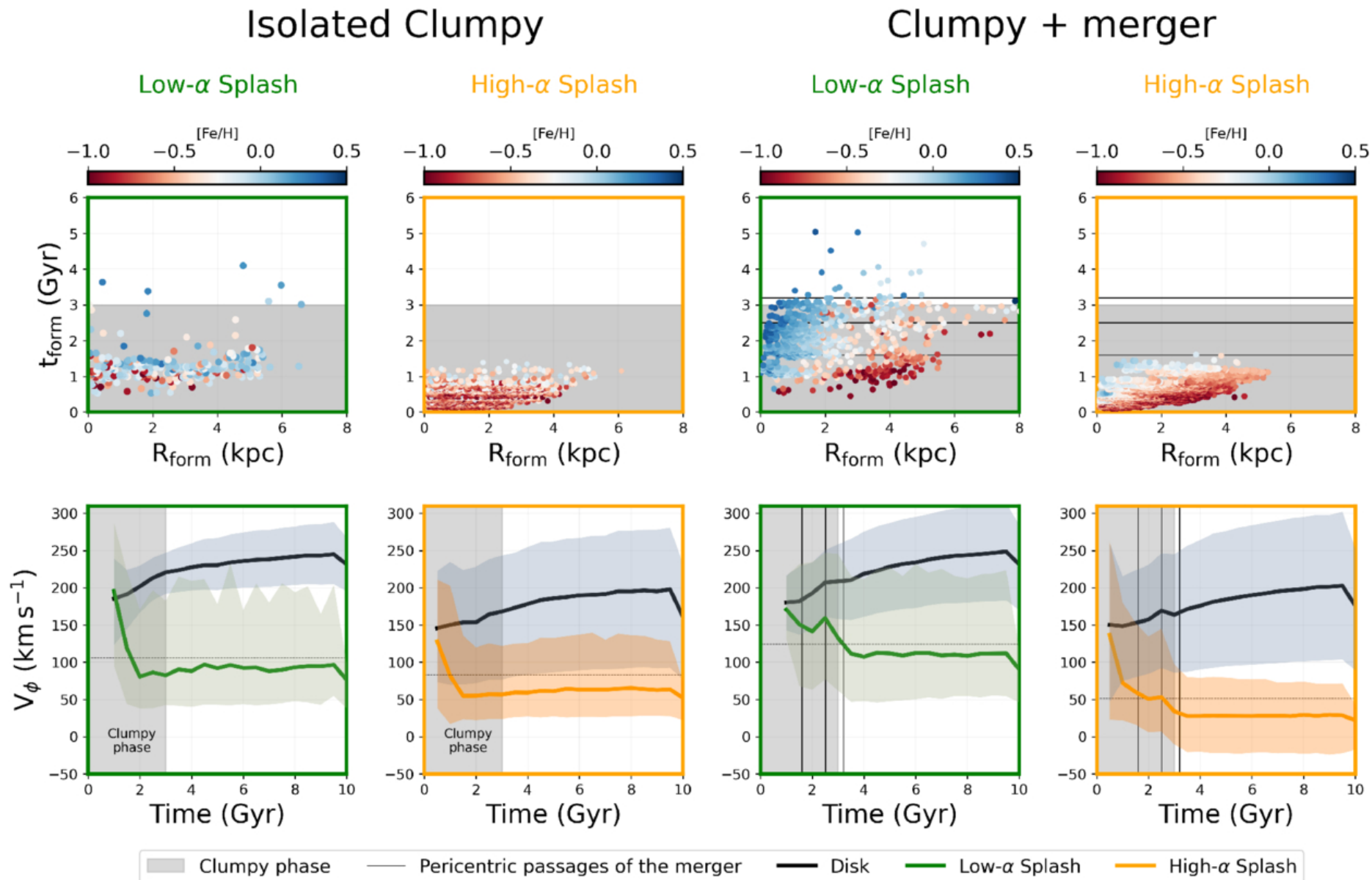
Figure 5. from Lais Borbolato et al 2026 Astrophys. J. Lett. 1008 doi:10.3847/2041-8213/ae9605 https://dx.doi.org/10.3847/2041-8213/ae9605 © 2026. The Author(s). Published by the American Astronomical Society.
