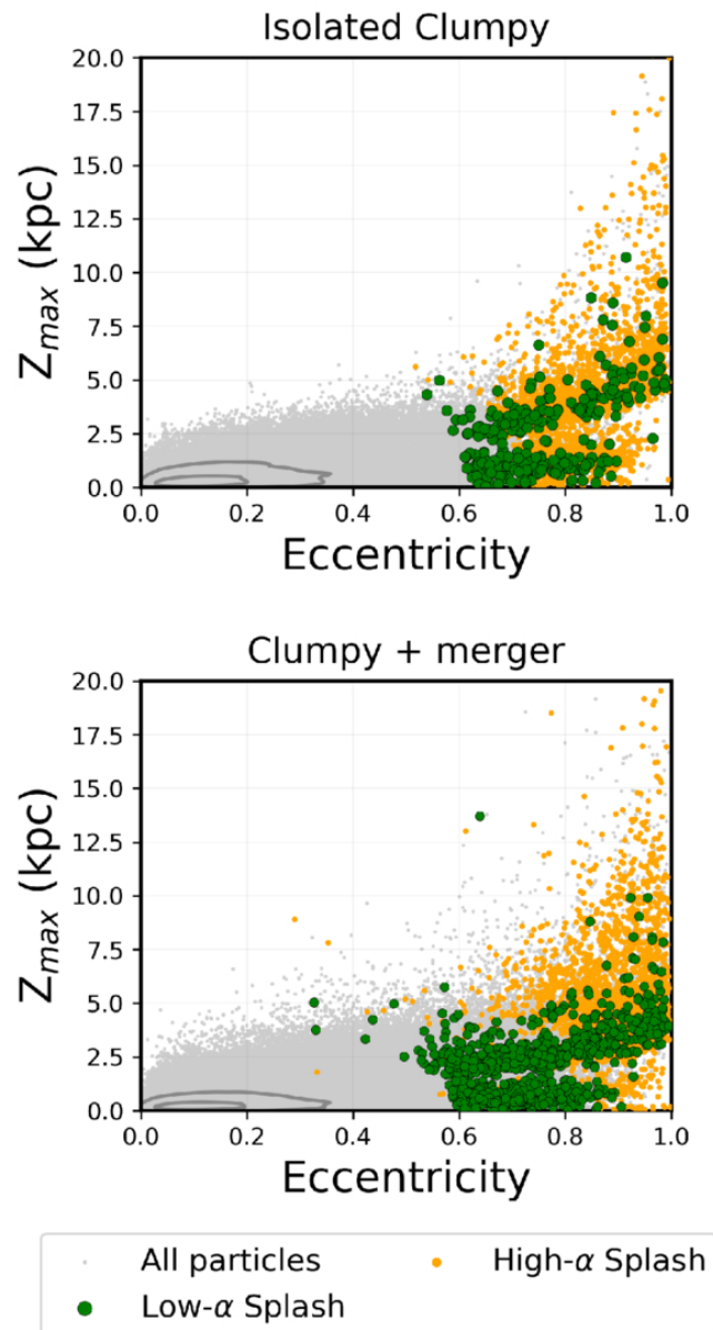
Figure 4. from Lais Borbolato et al 2026 Astrophys. J. Lett. 1008 doi:10.3847/2041-8213/ae9605 https://dx.doi.org/10.3847/2041-8213/ae9605 © 2026. The Author(s). Published by the American Astronomical Society.
