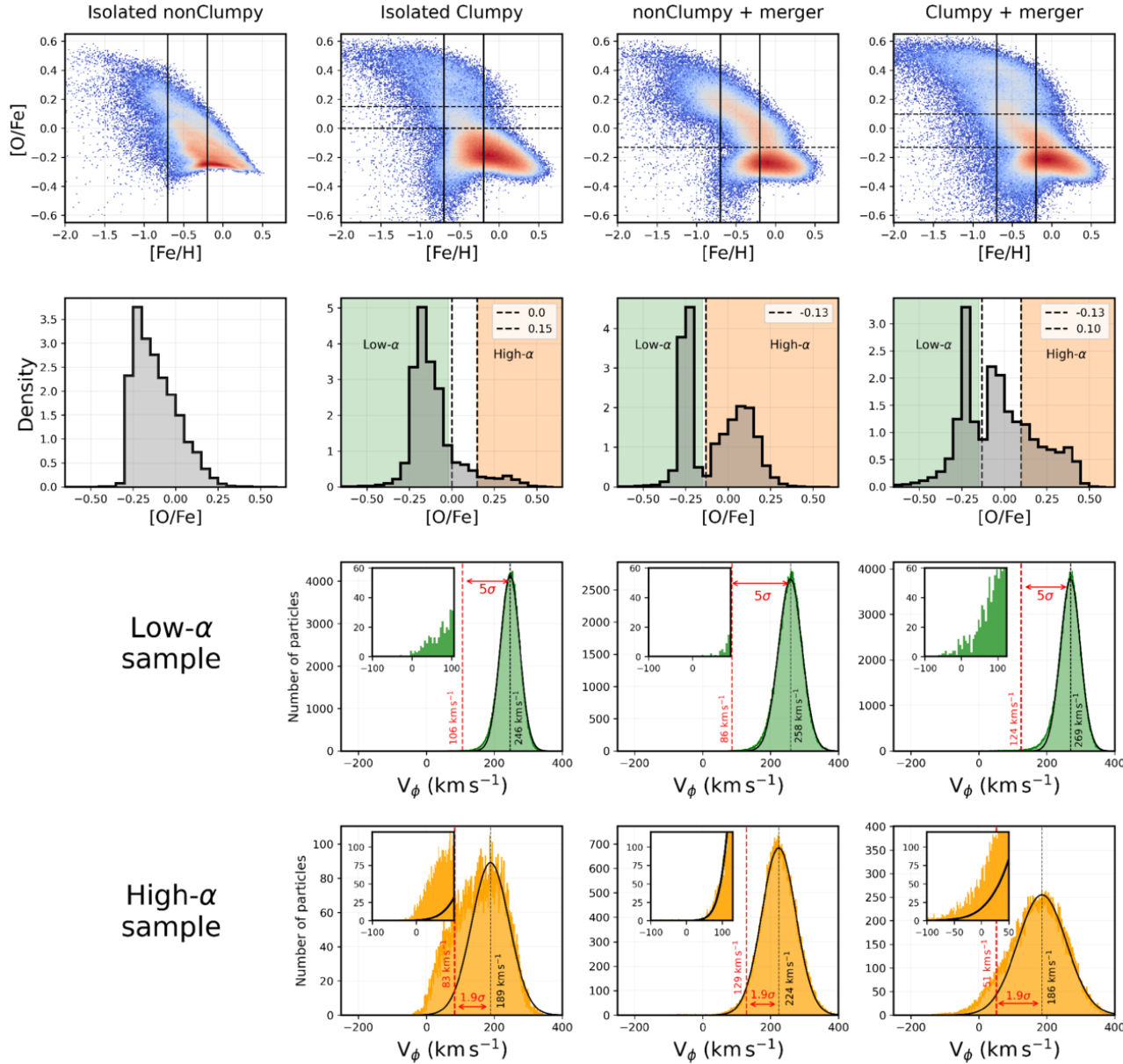
Figure 3. from Lais Borbolato et al 2026 Astrophys. J. Lett. 1008 doi:10.3847/2041-8213/ae9605 https://dx.doi.org/10.3847/2041-8213/ae9605 © 2026. The Author(s). Published by the American Astronomical Society.
