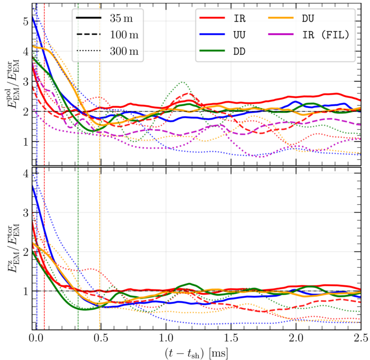
Figure 4. from Harry Ho-Yin Ng et al 2026 Astrophys. J. Lett. 1008 doi:10.3847/2041-8213/ae9601 https://dx.doi.org/10.3847/2041-8213/ae9601 © 2026. The Author(s). Published by the American Astronomical Society.
