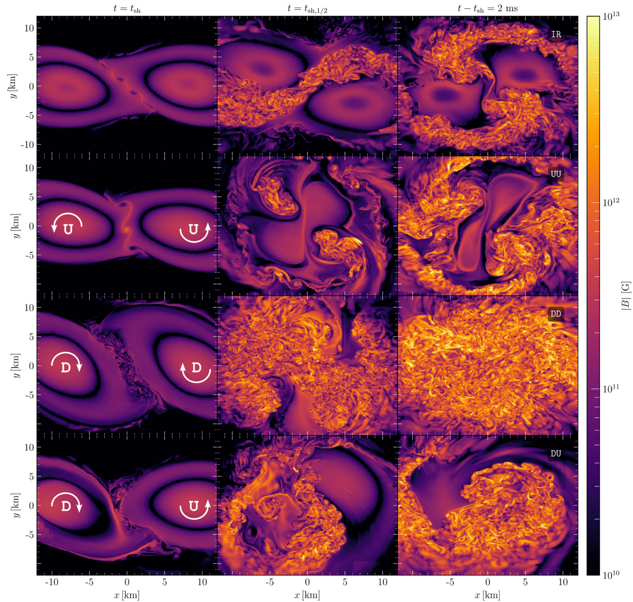
Figure 2. from Harry Ho-Yin Ng et al 2026 Astrophys. J. Lett. 1008 doi:10.3847/2041-8213/ae9601 https://dx.doi.org/10.3847/2041-8213/ae9601 © 2026. The Author(s). Published by the American Astronomical Society.
