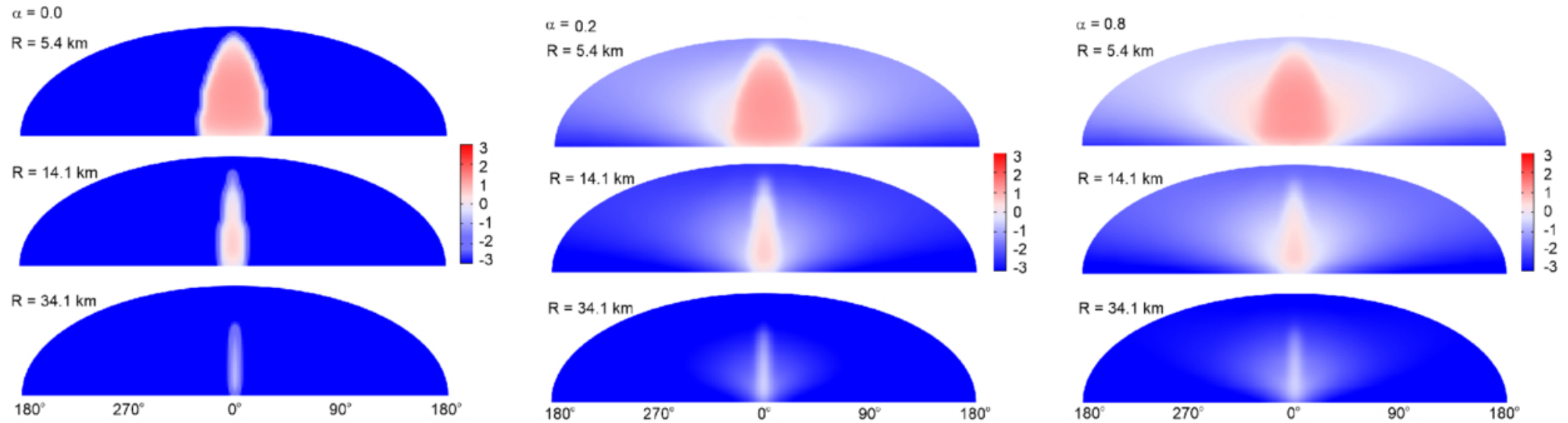
Figure 5. from Miroslav Kocifaj et al 2026 Astrophys. J. Lett. 1008 doi:10.3847/2041-8213/ae9551 https://dx.doi.org/10.3847/2041-8213/ae9551 © 2026. The Author(s). Published by the American Astronomical Society.
