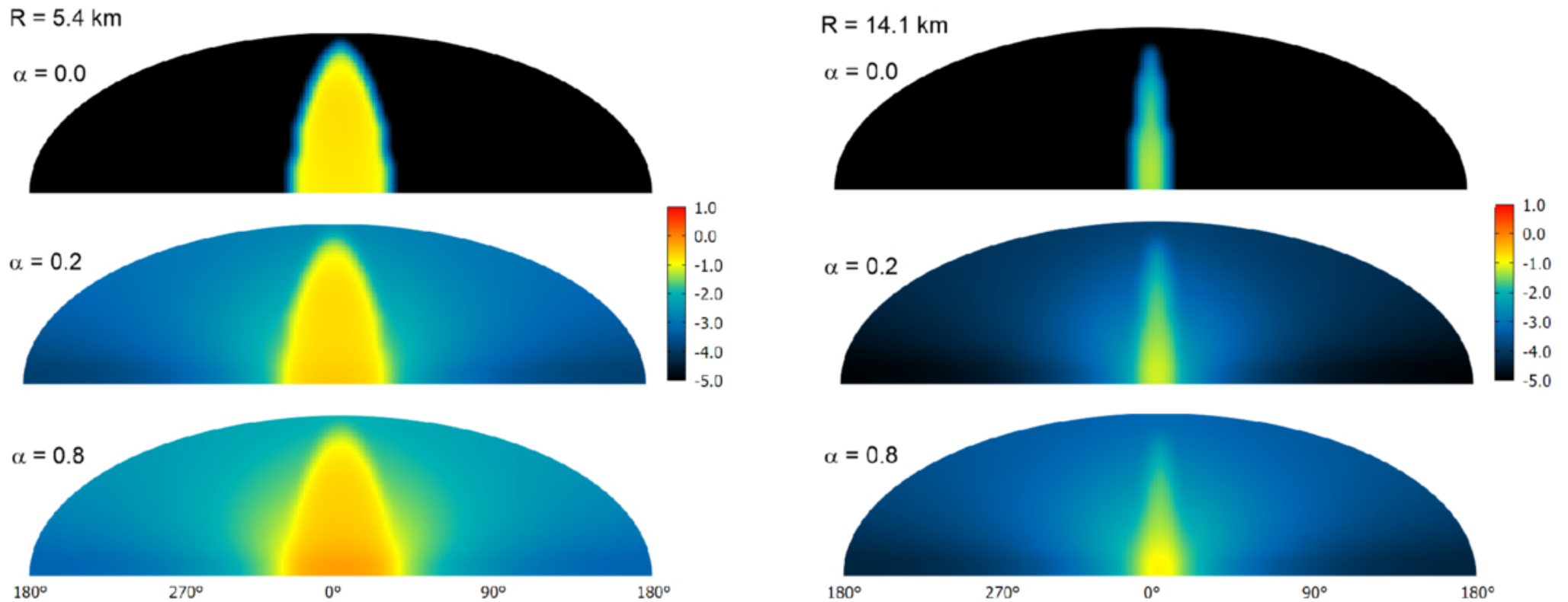
Figure 2. from Miroslav Kocifaj et al 2026 Astrophys. J. Lett. 1008 doi:10.3847/2041-8213/ae9551 https://dx.doi.org/10.3847/2041-8213/ae9551 © 2026. The Author(s). Published by the American Astronomical Society.
