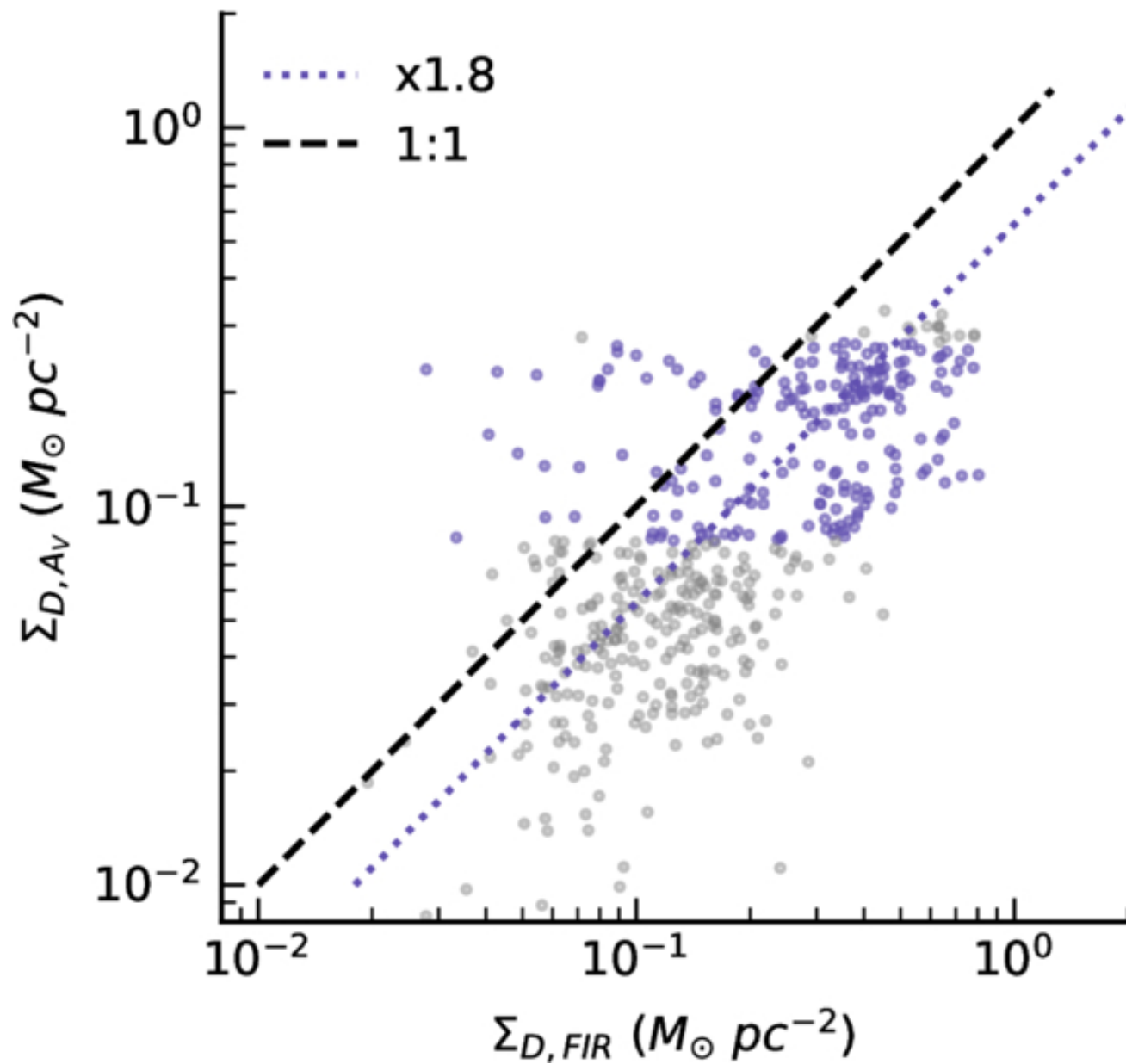
Figure 1. from Christina W. Lindberg et al 2026 Astrophys. J. Lett. 1007 doi:10.3847/2041-8213/ae954f https://dx.doi.org/10.3847/2041-8213/ae954f © 2026. The Author(s). Published by the American Astronomical Society.
