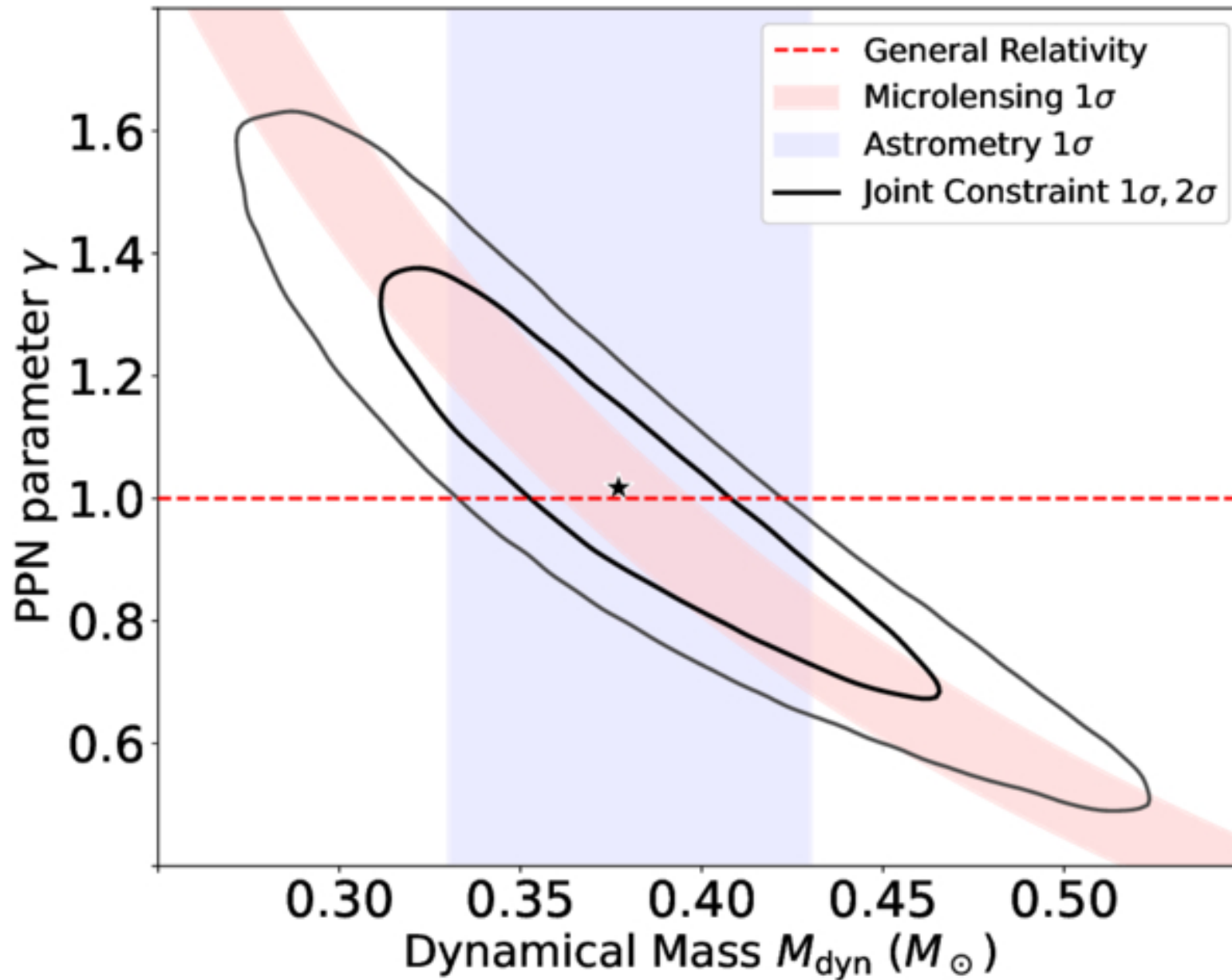
Figure 3. from Xinyang Jin et al 2026 Astrophys. J. Lett. 1008 doi:10.3847/2041-8213/ae954b https://dx.doi.org/10.3847/2041-8213/ae954b © 2026. The Author(s). Published by the American Astronomical Society.
