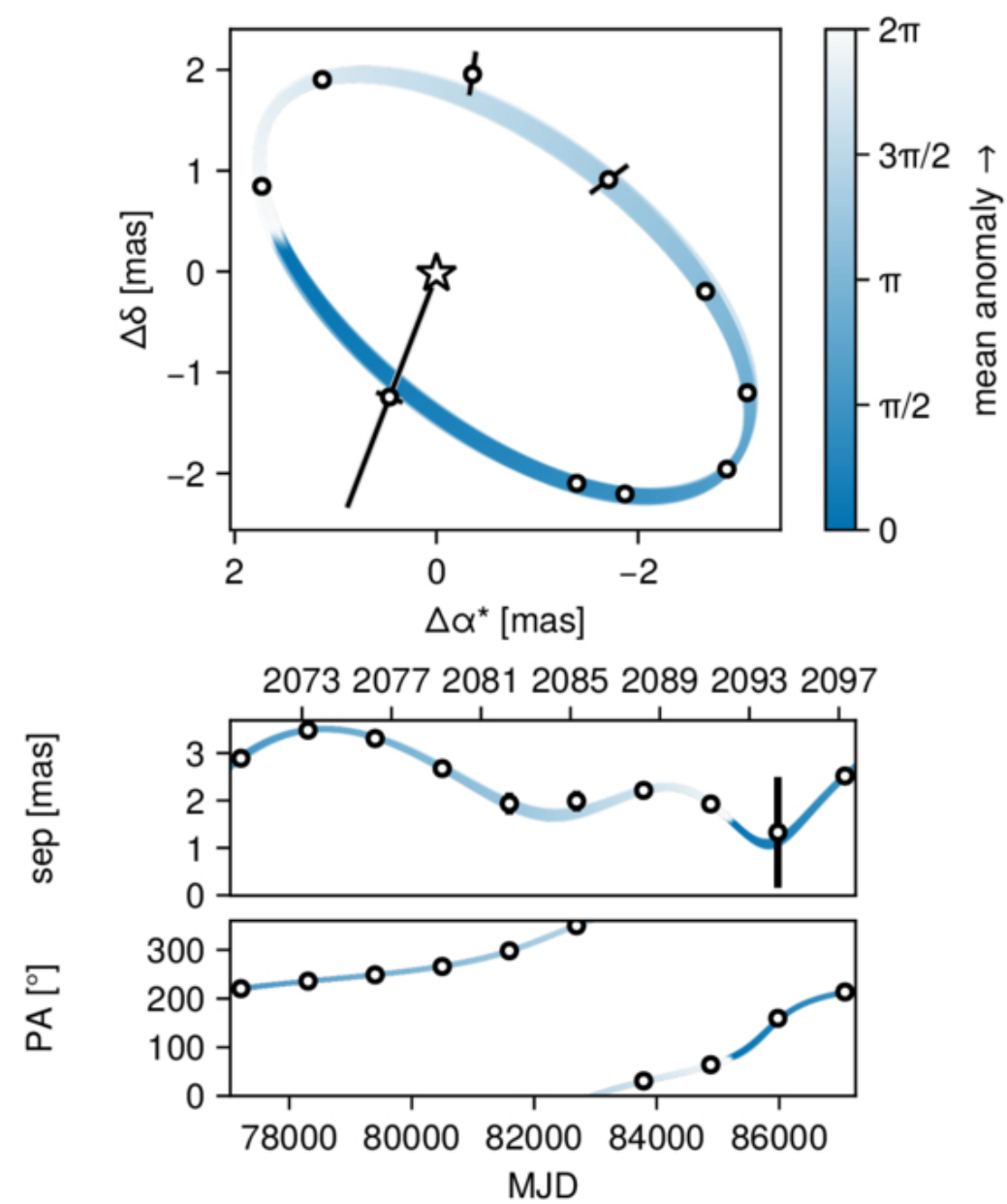
Figure 2. from Xinyang Jin et al 2026 Astrophys. J. Lett. 1008 doi:10.3847/2041-8213/ae954b https://dx.doi.org/10.3847/2041-8213/ae954b © 2026. The Author(s). Published by the American Astronomical Society.
