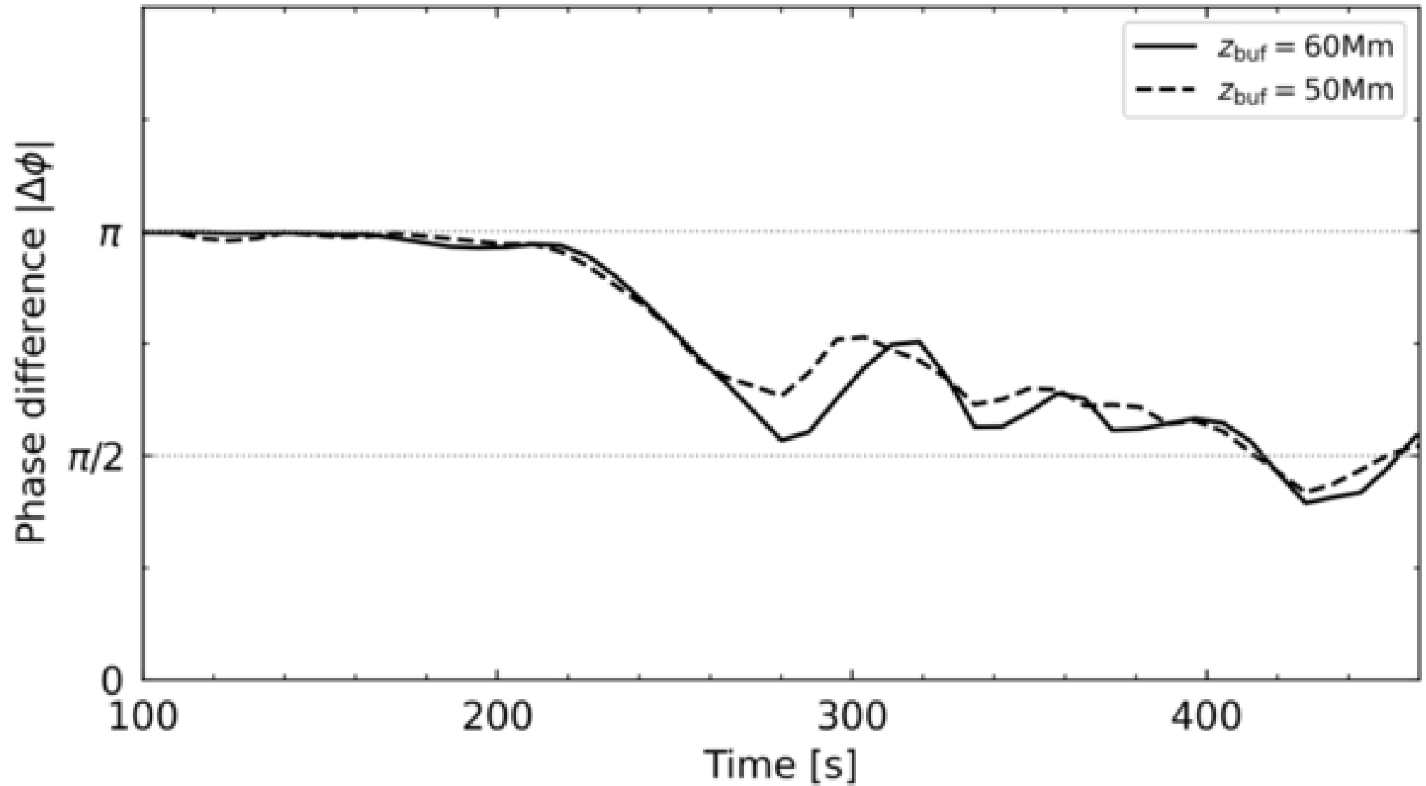
Figure 8. from Mingzhe Guo et al 2026 Astrophys. J. Lett. 1007 doi:10.3847/2041-8213/ae9474 https://dx.doi.org/10.3847/2041-8213/ae9474 © 2026. The Author(s). Published by the American Astronomical Society.
