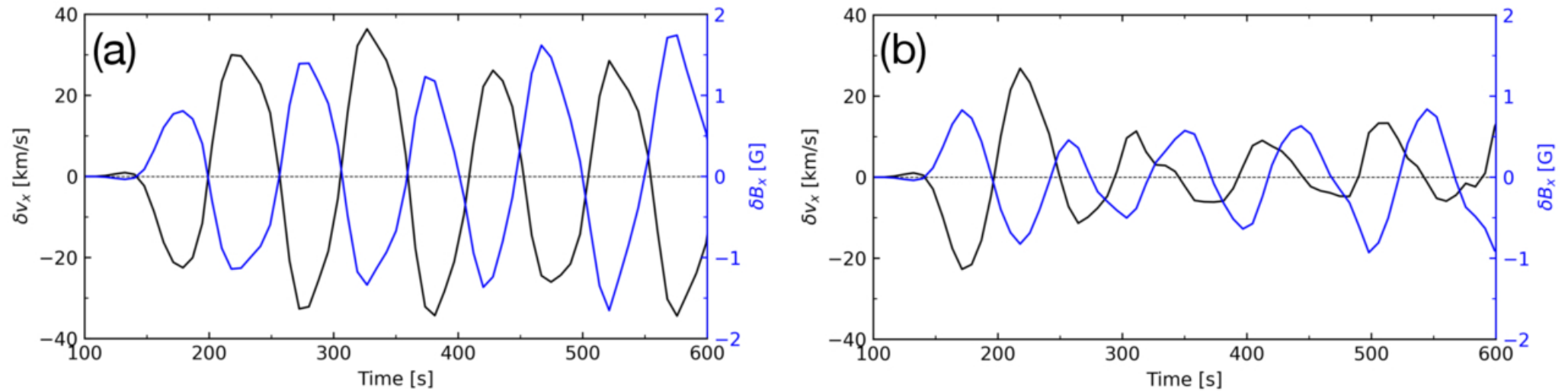
Figure 7. from Mingzhe Guo et al 2026 Astrophys. J. Lett. 1007 doi:10.3847/2041-8213/ae9474 https://dx.doi.org/10.3847/2041-8213/ae9474 © 2026. The Author(s). Published by the American Astronomical Society.
