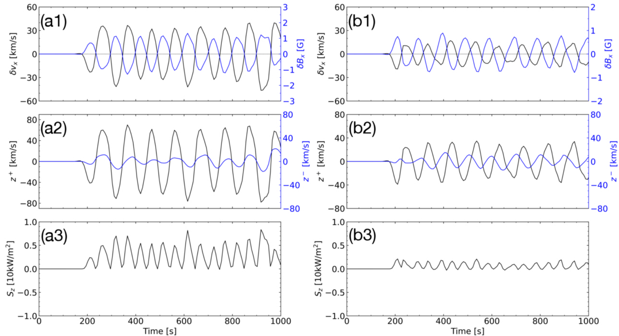
Figure 6. from Mingzhe Guo et al 2026 Astrophys. J. Lett. 1007 doi:10.3847/2041-8213/ae9474 https://dx.doi.org/10.3847/2041-8213/ae9474 © 2026. The Author(s). Published by the American Astronomical Society.
