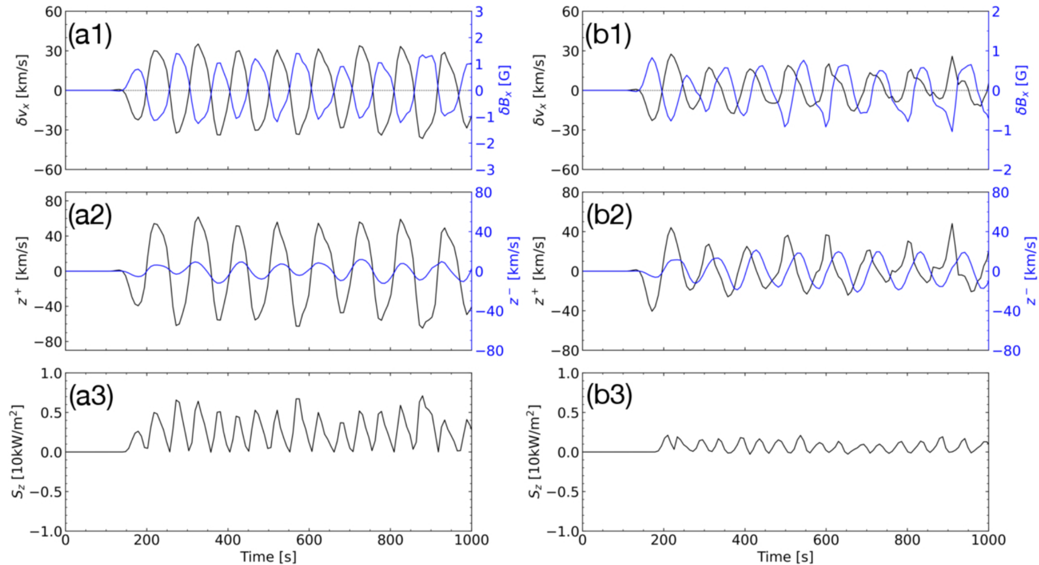
Figure 4. from Mingzhe Guo et al 2026 Astrophys. J. Lett. 1007 doi:10.3847/2041-8213/ae9474 https://dx.doi.org/10.3847/2041-8213/ae9474 © 2026. The Author(s). Published by the American Astronomical Society.
