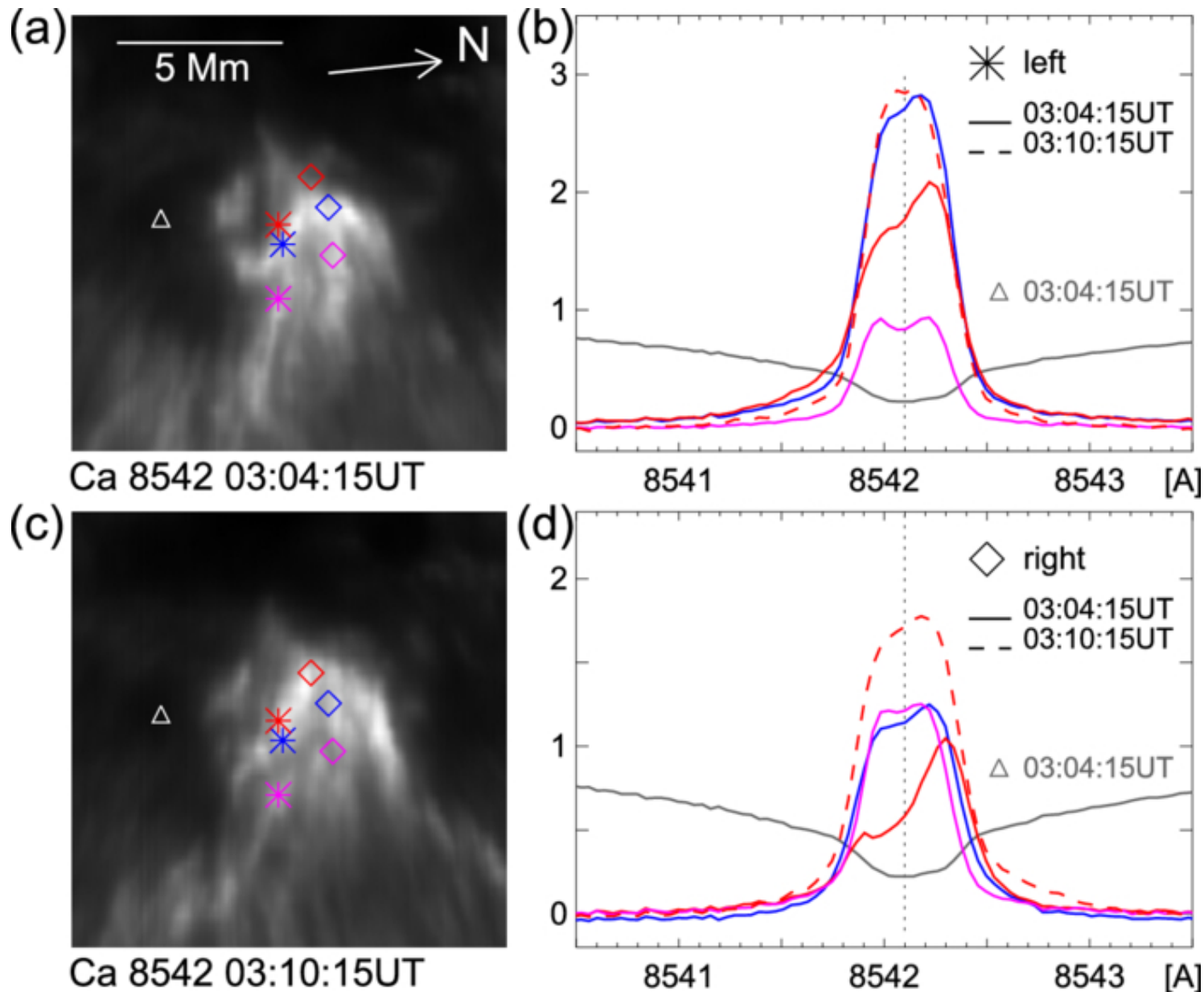
Figure 5. from Ayumi Asai et al 2026 Astrophys. J. Lett. 1008 doi:10.3847/2041-8213/ae946f https://dx.doi.org/10.3847/2041-8213/ae946f © 2026. The Author(s). Published by the American Astronomical Society.
