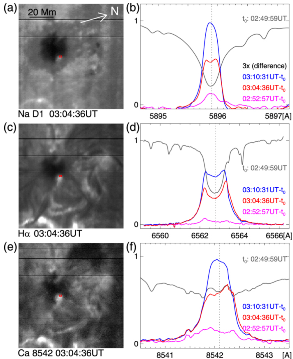
Figure 4. from Ayumi Asai et al 2026 Astrophys. J. Lett. 1008 doi:10.3847/2041-8213/ae946f https://dx.doi.org/10.3847/2041-8213/ae946f © 2026. The Author(s). Published by the American Astronomical Society.
