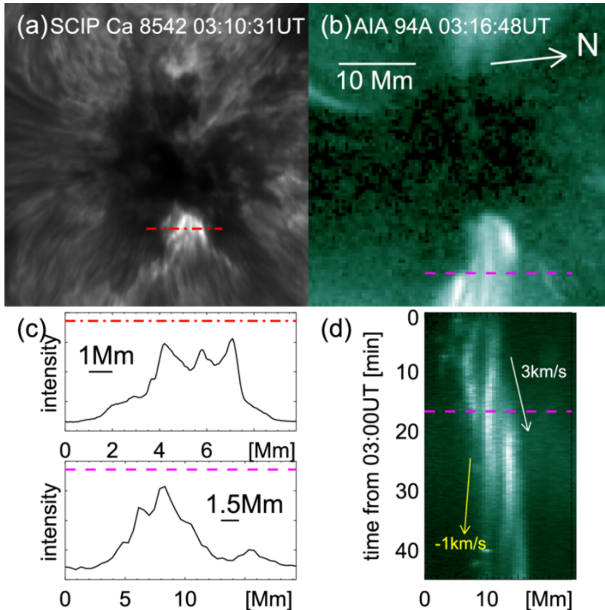
Figure 3. from Ayumi Asai et al 2026 Astrophys. J. Lett. 1008 doi:10.3847/2041-8213/ae946f https://dx.doi.org/10.3847/2041-8213/ae946f © 2026. The Author(s). Published by the American Astronomical Society.
