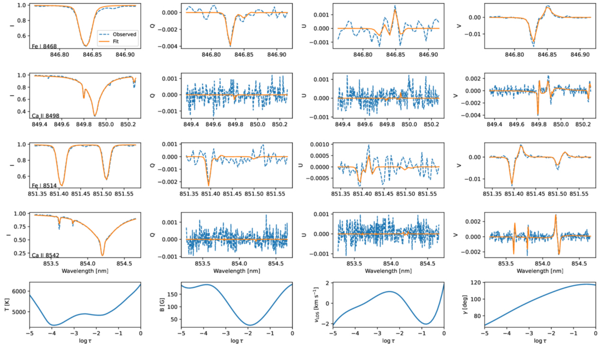
Figure 6. from Ryan J. Campbell et al 2026 Astrophys. J. Lett. 1008 doi:10.3847/2041-8213/ae946e https://dx.doi.org/10.3847/2041-8213/ae946e © 2026. The Author(s). Published by the American Astronomical Society.
