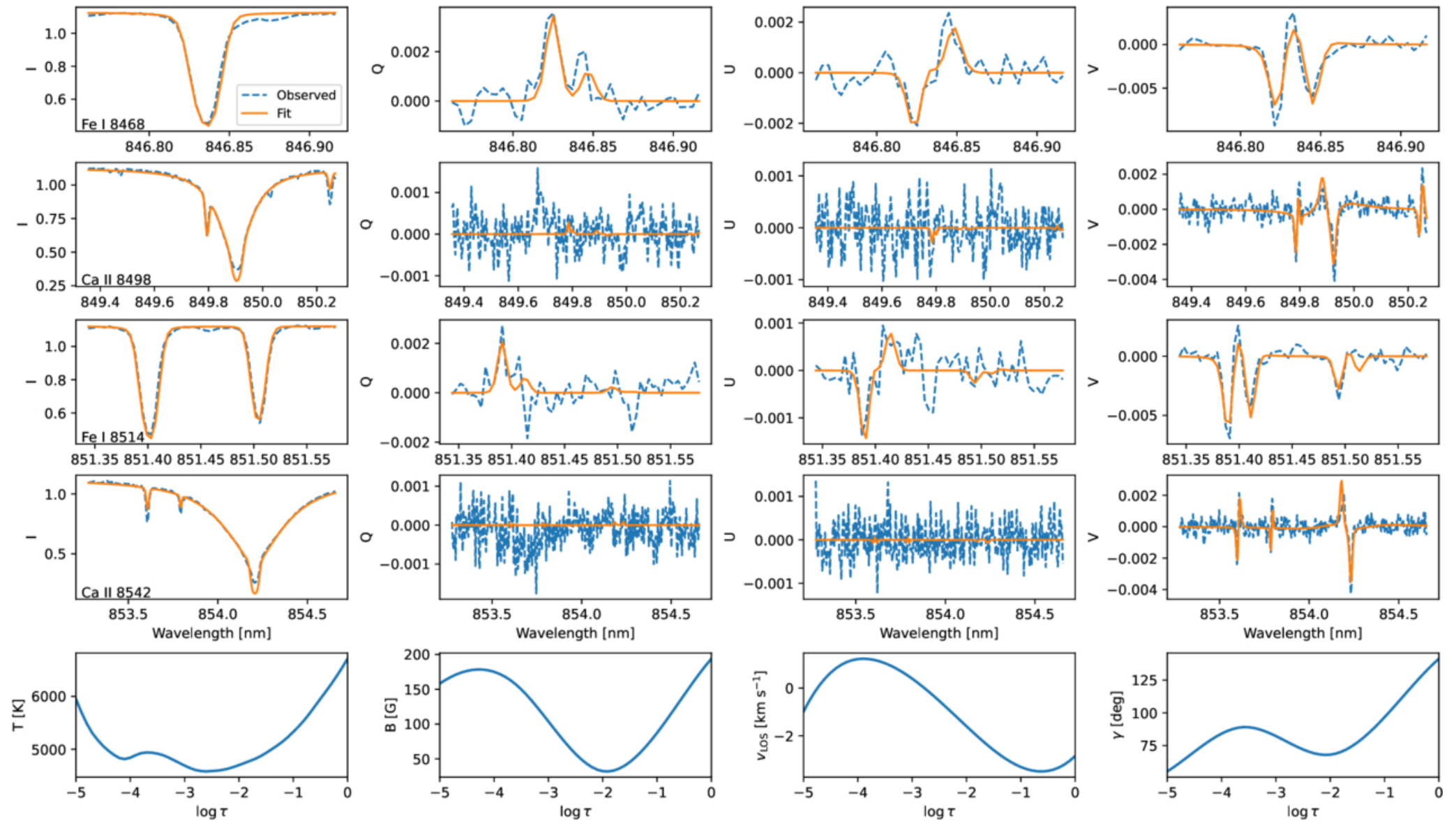
Figure 5. from Ryan J. Campbell et al 2026 Astrophys. J. Lett. 1008 doi:10.3847/2041-8213/ae946e https://dx.doi.org/10.3847/2041-8213/ae946e © 2026. The Author(s). Published by the American Astronomical Society.
