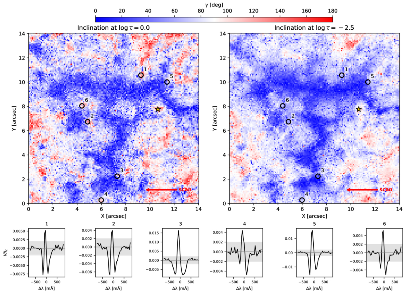
Figure 4. from Ryan J. Campbell et al 2026 Astrophys. J. Lett. 1008 doi:10.3847/2041-8213/ae946e https://dx.doi.org/10.3847/2041-8213/ae946e © 2026. The Author(s). Published by the American Astronomical Society.
