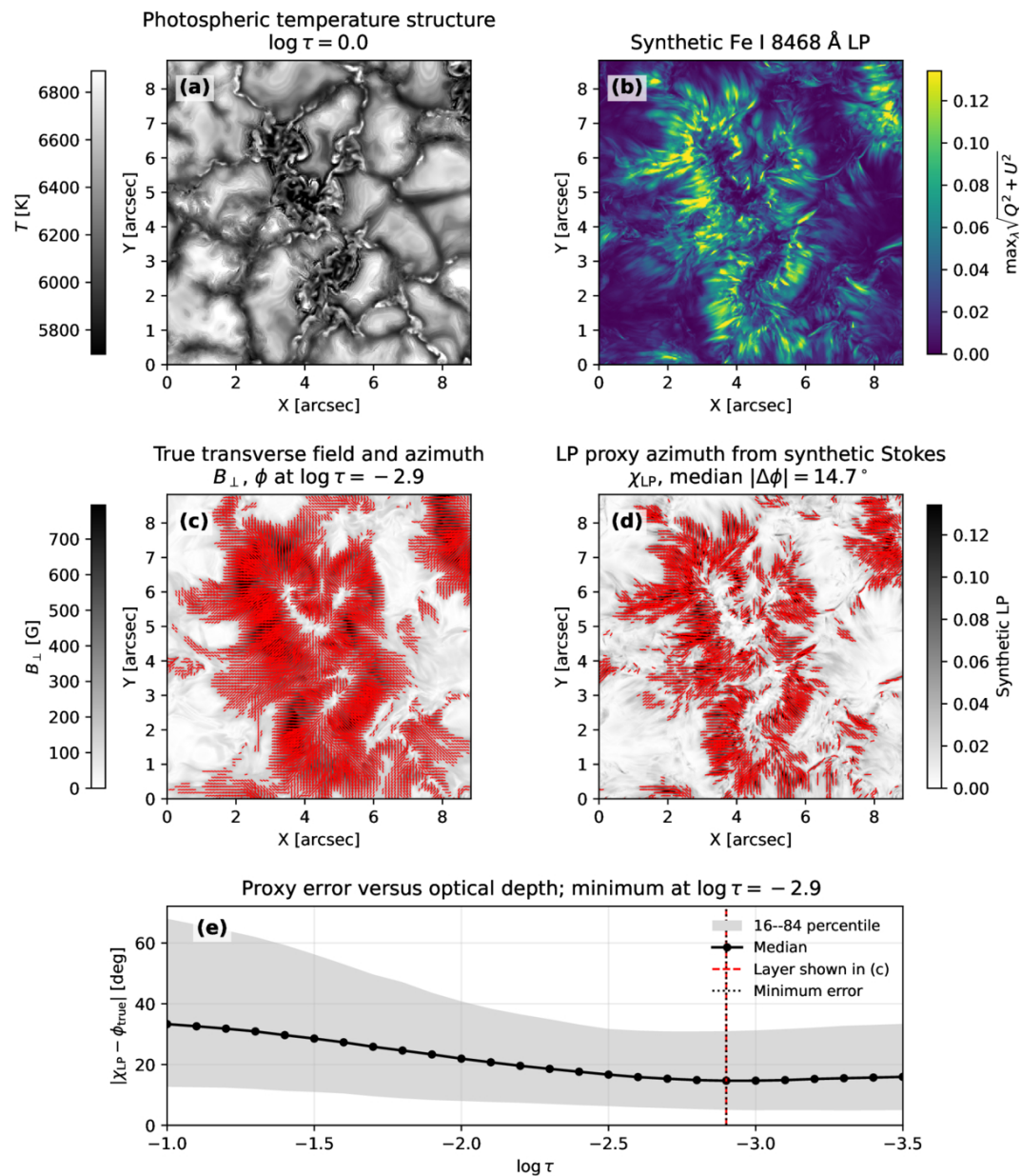
Figure 3. from Ryan J. Campbell et al 2026 Astrophys. J. Lett. 1008 doi:10.3847/2041-8213/ae946e https://dx.doi.org/10.3847/2041-8213/ae946e © 2026. The Author(s). Published by the American Astronomical Society.
