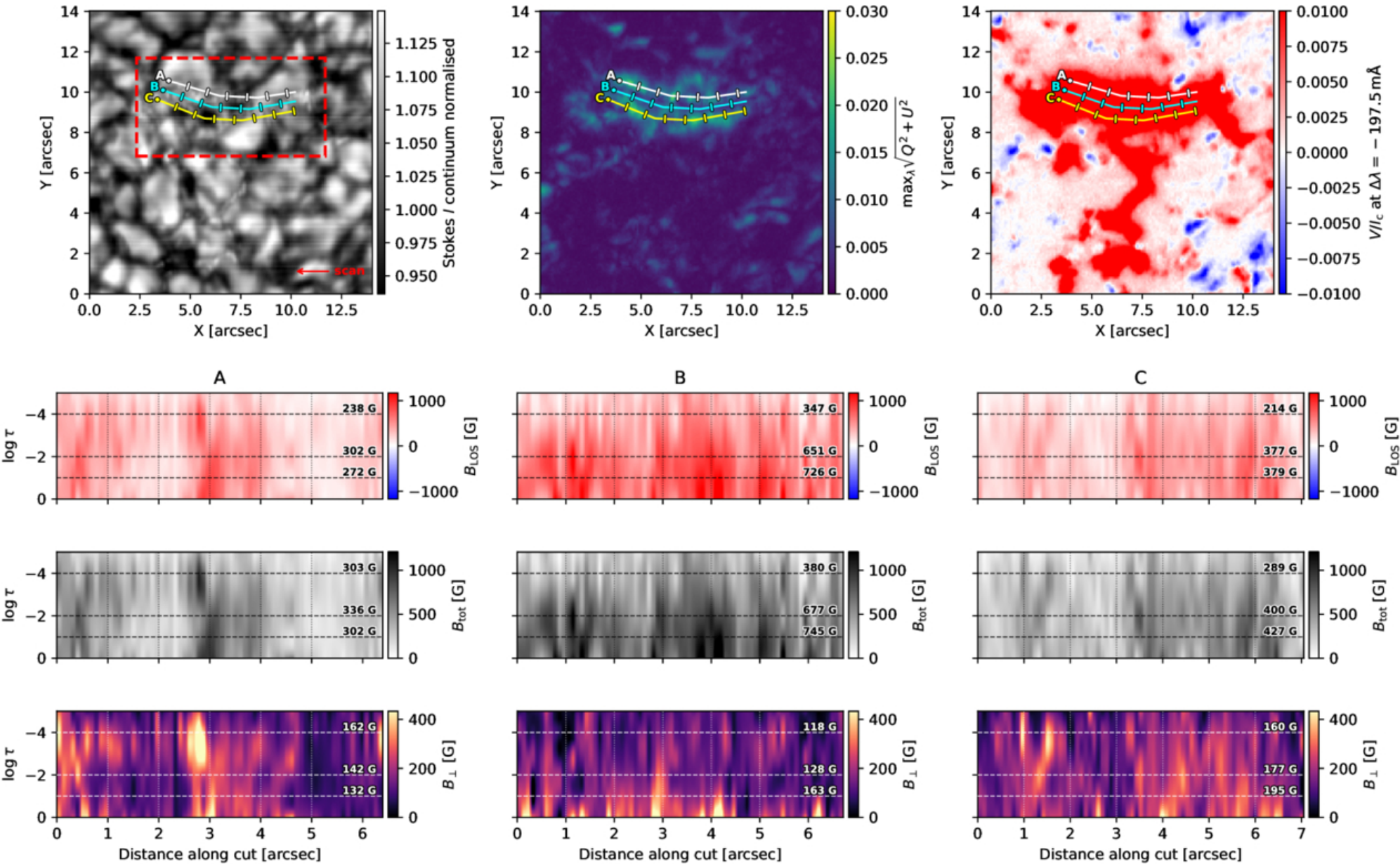
Figure 1. from Ryan J. Campbell et al 2026 Astrophys. J. Lett. 1008 doi:10.3847/2041-8213/ae946e https://dx.doi.org/10.3847/2041-8213/ae946e © 2026. The Author(s). Published by the American Astronomical Society.
