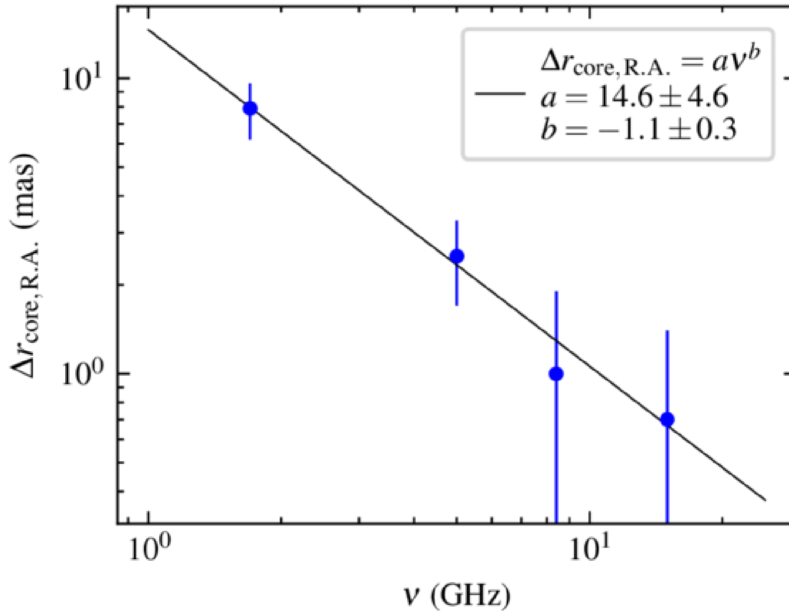
Figure 4. from Xi Yan et al 2026 Astrophys. J. Lett. 1007 doi:10.3847/2041-8213/ae93b4 https://dx.doi.org/10.3847/2041-8213/ae93b4 © 2026. The Author(s). Published by the American Astronomical Society.
