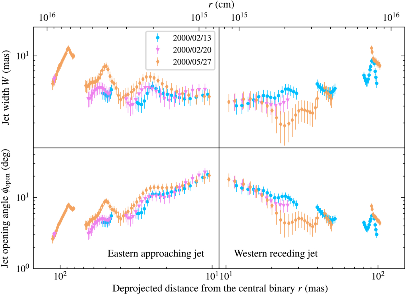
Figure 3. from Xi Yan et al 2026 Astrophys. J. Lett. 1007 doi:10.3847/2041-8213/ae93b4 https://dx.doi.org/10.3847/2041-8213/ae93b4 © 2026. The Author(s). Published by the American Astronomical Society.
