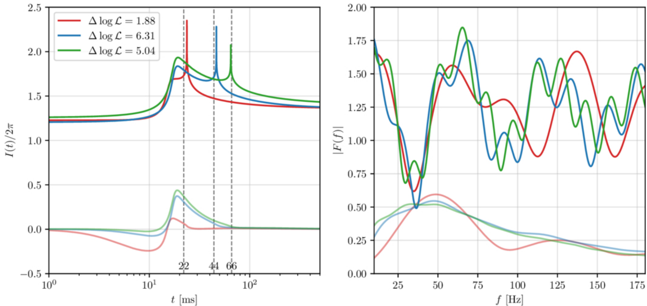
Figure A2. from Srashti Goyal et al 2026 Astrophys. J. Lett. 1008 doi:10.3847/2041-8213/ae93b1 https://dx.doi.org/10.3847/2041-8213/ae93b1 © 2026. The Author(s). Published by the American Astronomical Society.
