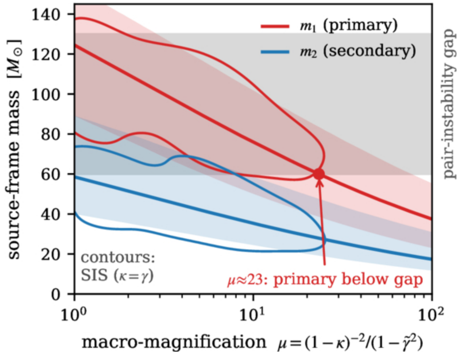
Figure B2. from Srashti Goyal et al 2026 Astrophys. J. Lett. 1008 doi:10.3847/2041-8213/ae93b1 https://dx.doi.org/10.3847/2041-8213/ae93b1 © 2026. The Author(s). Published by the American Astronomical Society.
