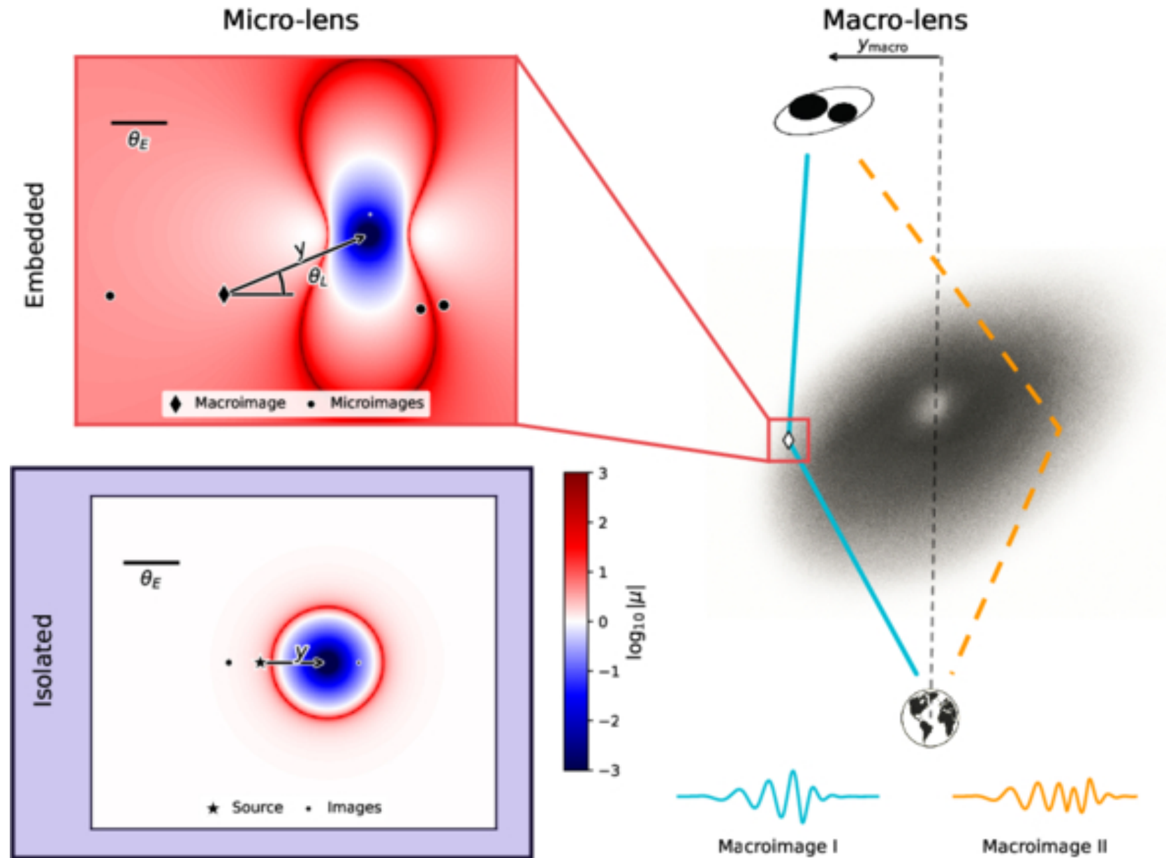
Figure 1. from Srashti Goyal et al 2026 Astrophys. J. Lett. 1008 doi:10.3847/2041-8213/ae93b1 https://dx.doi.org/10.3847/2041-8213/ae93b1 © 2026. The Author(s). Published by the American Astronomical Society.
