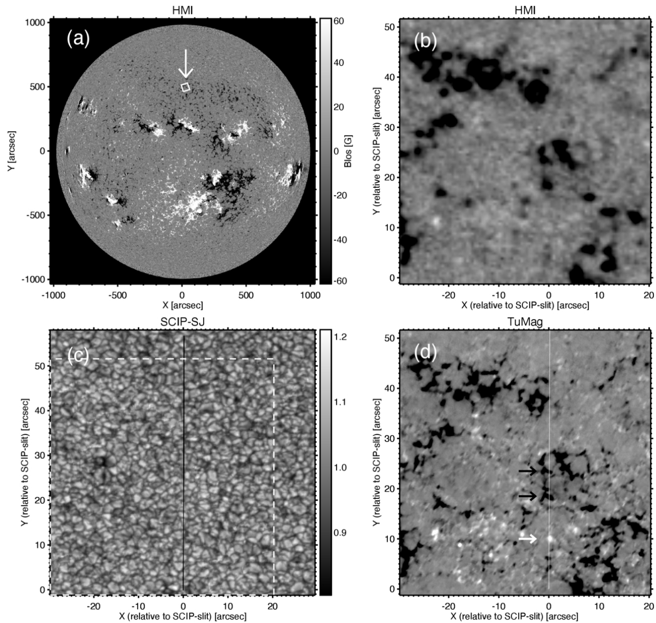
Figure 1. from Takayoshi Oba et al 2026 Astrophys. J. Lett. 1008 doi:10.3847/2041-8213/ae9398 https://dx.doi.org/10.3847/2041-8213/ae9398 © 2026. The Author(s). Published by the American Astronomical Society.
